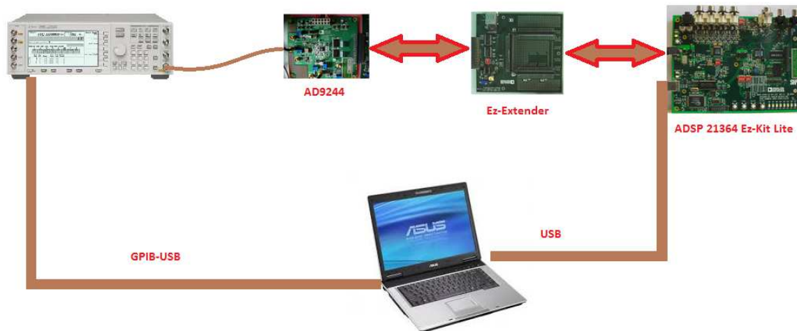
Fig. 2. Measurement station.
