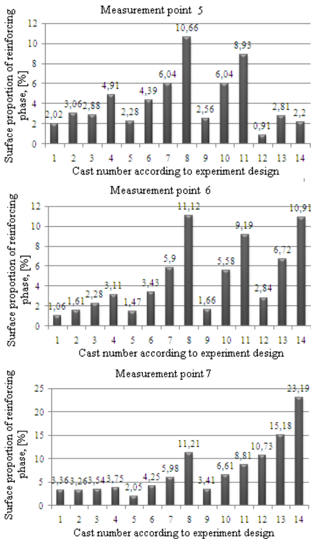
Fig. 8. Distribution of reinforcing phase along vertical axis on the individual measurement points (1÷7) in composite casts
