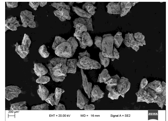
Fig. 1. Particles CrFe30C8 used in tests: a) 100 \mu\text{m} , b) 200 \mu\text{m} , c) 315 \mu\text{m}
