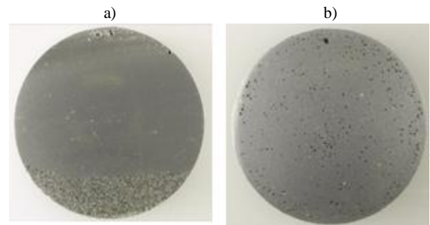
Fig. 6. Example of macrostructure of composite samples: a) without electromagnetic field, b) with electromagnetic field
