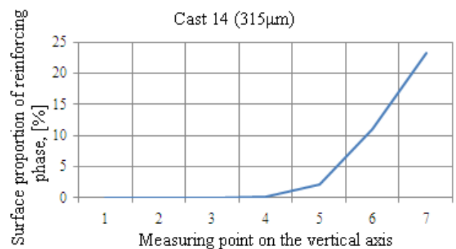
Fig. 7. Gravity segregation of reinforcement phase along height of cast equal to the diameter of the casting trial
