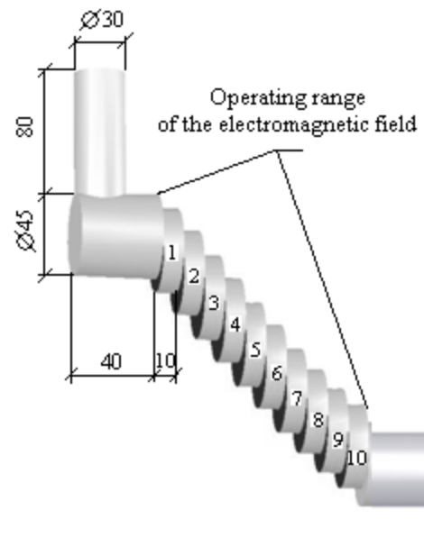
Fig. 3. Preparation method of samples to metallographic testing: b) method of samples excision used in tests (1÷10 samples number )
