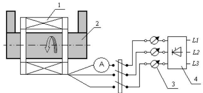
Fig. 2. Diagram of stand to generation of electromagnetic field: 1 – inductor, 2 – shell mould, 3 – autotransformer, 4 - inverter
