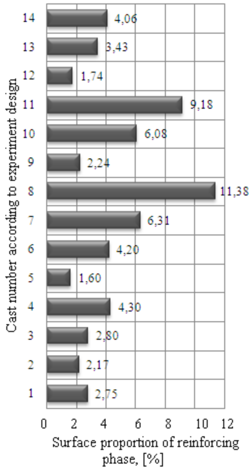
Fig. 5. Surface proportion of reinforcing phase in tests composite casts
