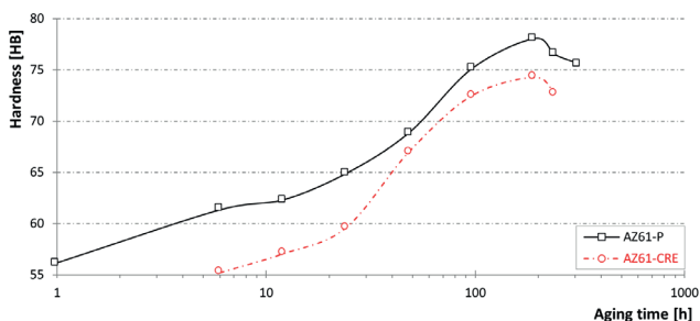
Fig. 4. Hardness of AZ61 and AZ61-P-CRE profiles after solution heat treatment and aging
