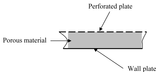
Fig. 2. Composition of the used liner.
