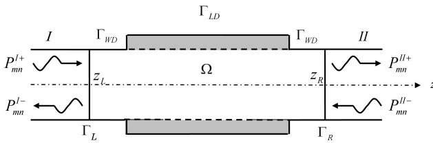
Fig. 1. The calculation domain.
