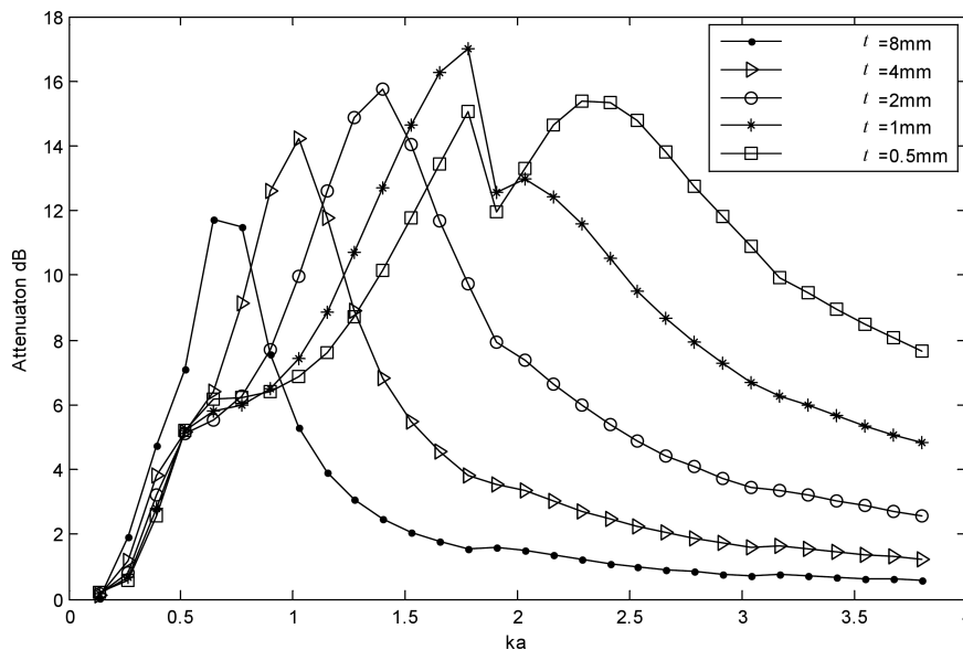
Fig. 6. Effect of the thickness t [mm] of the perforated plate on the acoustic power attenuation of the lined duct element.
