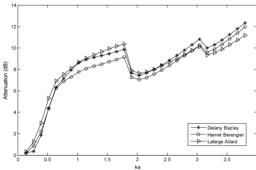
Fig. 3. Acoustic power attenuation of the studied duct for several porous materials models.
