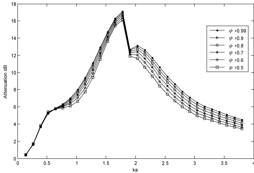
Fig. 9. Effect of the porosity \varphi of the porous material on the acoustic power attenuation of the lined duct element.
