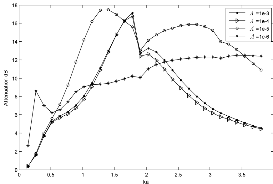
Fig. 12. Effect of the characteristic viscous length \Lambda [m] of the porous material on the acoustic power attenuation of the lined duct element.
