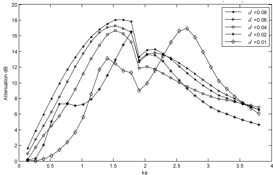
Fig. 8. Effect of the depth d [mm] of the porous material on the acoustic power attenuation of the lined duct element.
