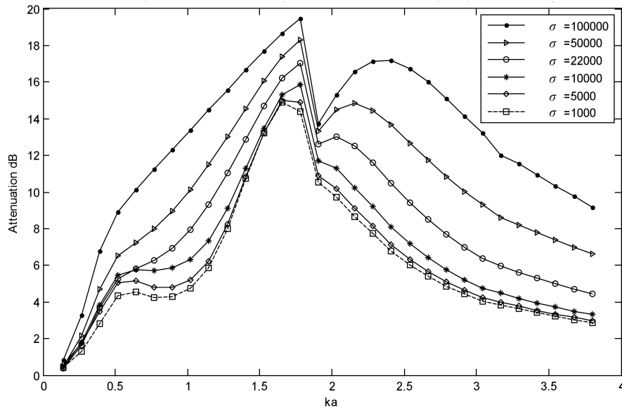
Fig. 7. Effect of the flow resistivity \sigma [ \text{Nm}^{-1}\text{s} ] of the porous material on the acoustic power attenuation of the lined duct element.
