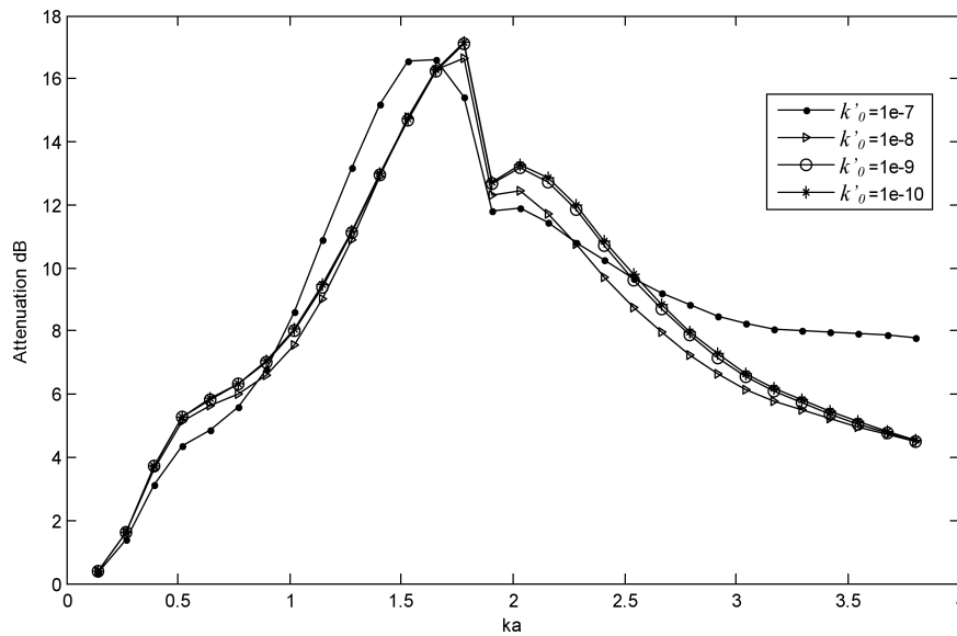
Fig. 11. Effect of the thermal permeability k'_0 [ \text{m}^2 ] of the porous material on the acoustic power attenuation of the lined duct element.
