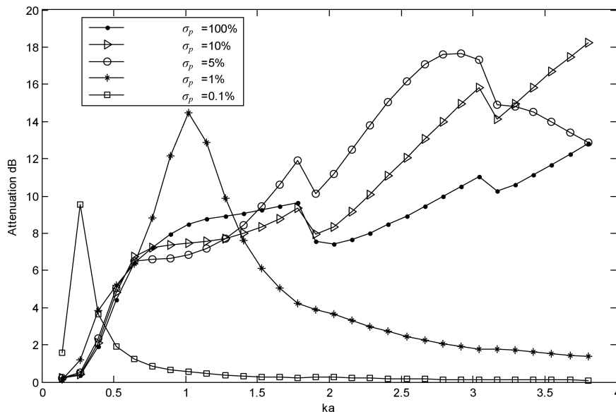
Fig. 5. Effect of the porosity \sigma_p [%] of the perforated plate on the acoustic power attenuation of the lined duct element.
