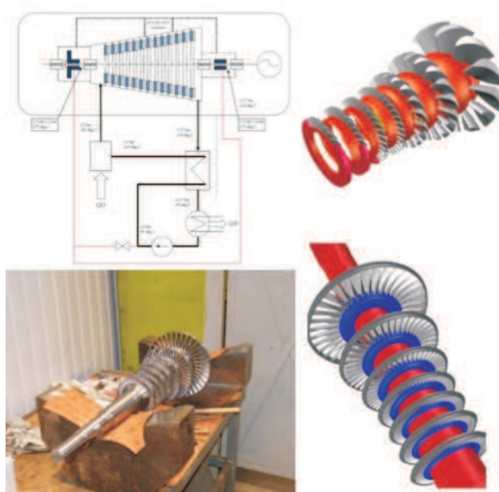
Figure 19: IMP PAN Laboratory: ORC turbogenerator (own solutions) for ARE; axial turbine 9000 rev/min, 100 kW.
