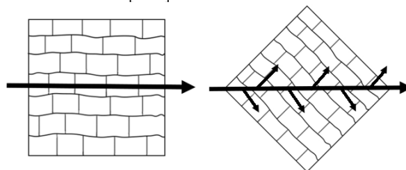
Fig. 1. Testing of anisotropic material – good direction of testing (left), direction with big attenuation (right) [2]
