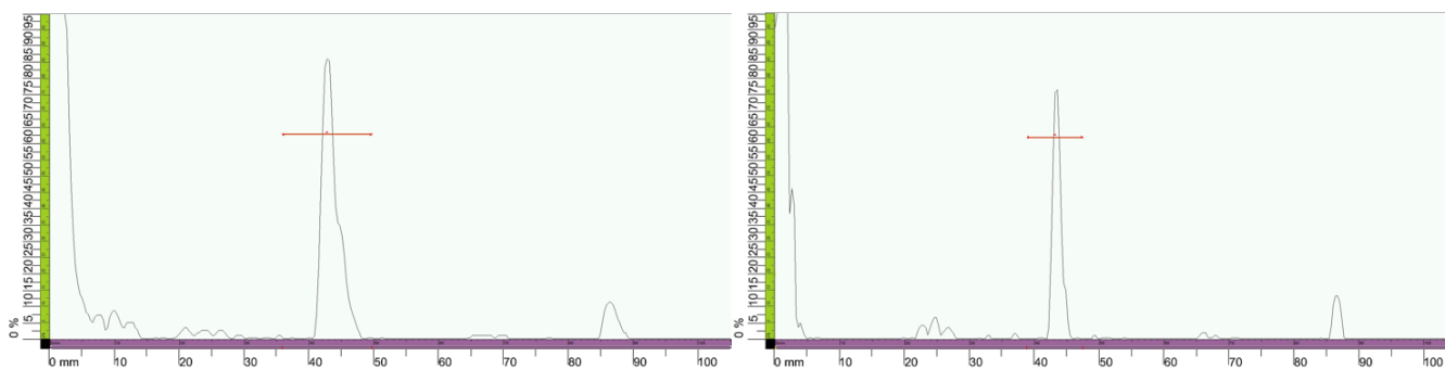
Fig. 3. Recording of evaluating attenuation of sample No. 2 (left – 3.5 MHz probe, right - 5 MHz probe frequency)
