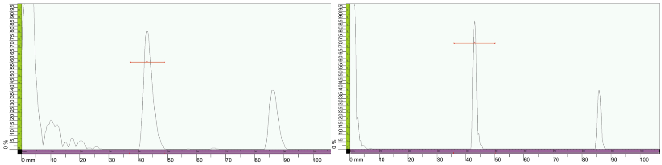
Fig. 4. Recording of evaluating attenuation of sample No. 3 (left – 3.5 MHz probe, right - 5 MHz probe frequency)
