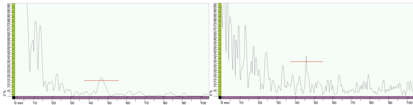
Fig. 2. Recording of evaluating attenuation of sample No. 1 (left – 3.5 MHz probe, right - 5 MHz probe frequency)
