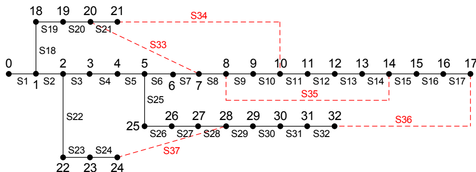
Fig. 8. IEEE 33-bus distribution system
