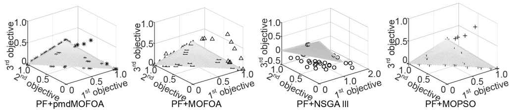
Fig. 6. Non-dominated solutions of each algorithm on the test function DTLZ1
