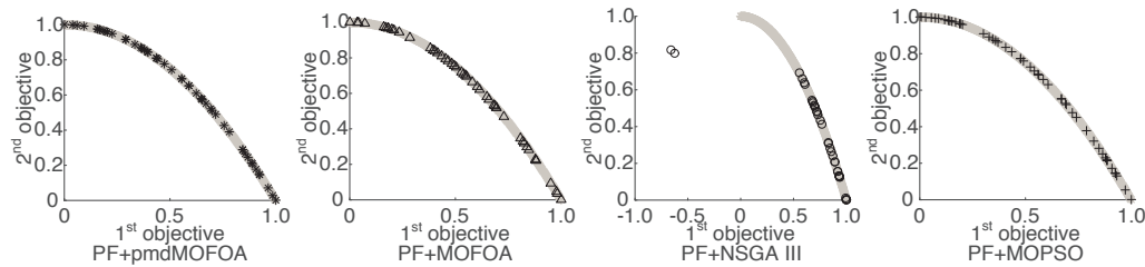
Fig. 4. Non-dominated solutions of each algorithm on the test function ZDT2
