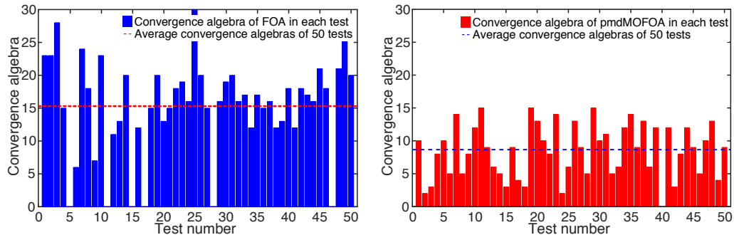
Fig. 2. Test results bar chart for 50 tests
