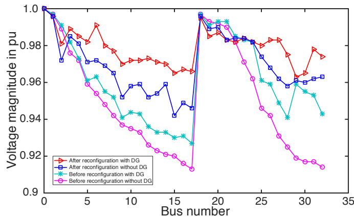
Fig. 10. Voltage distribution for the 33-bus system before and after using the proposed algorithm
