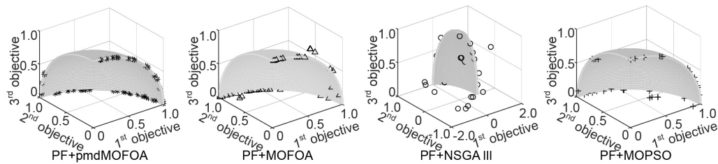
Fig. 7. Non-dominated solutions of each algorithm on the test function DTLZ2
