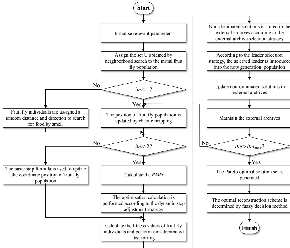
Fig. 1. Flow chart of distribution network reconfiguration
