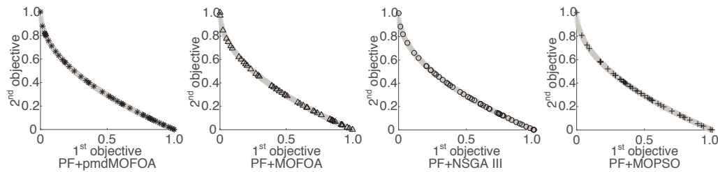
Fig. 3. Non-dominated solutions of each algorithm on the test function ZDT1
