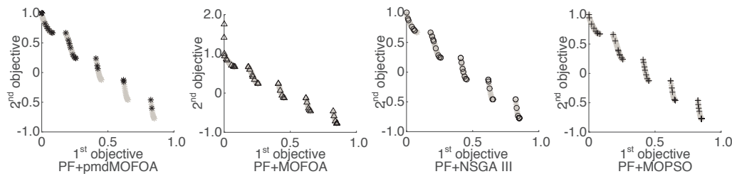
Fig. 5. Non-dominated solutions of each algorithm on the test function ZDT3
