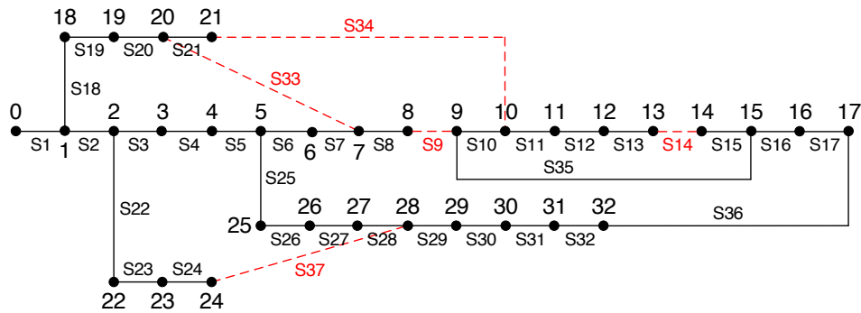
Fig. 9. IEEE 33-bus distribution system after reconfiguration
