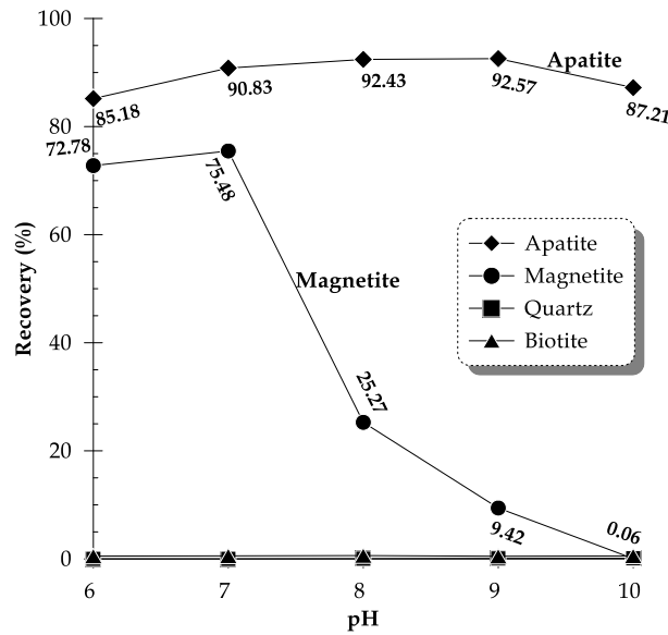
Fig. 2. The effect of pH on the single minerals flotation (Pulp density: 10%, fatty acid dosage: 200 mg/dm 3 , surfactant dosage: 0 mg/dm 3 , temperature: 25°C, flotation time: 3 min, and pH 6.0-10.0)
