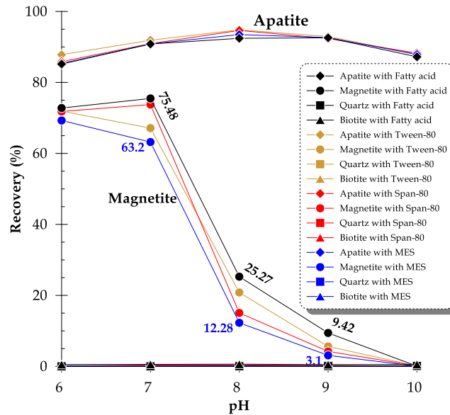
Fig. 4. The effect of the surfactant under various pH on the single minerals flotation (Pulp density: 10%, fatty acid dosage: 200 mg/dm 3 , surfactant dosage: 15 mg/dm 3 , temperature: 25°C, flotation time: 3 min, and pH 6.0-10.0)
