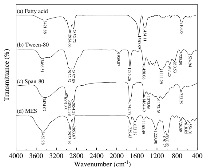
Fig. 7. FTIR spectra of the reagents at pH 8 and 25°C
