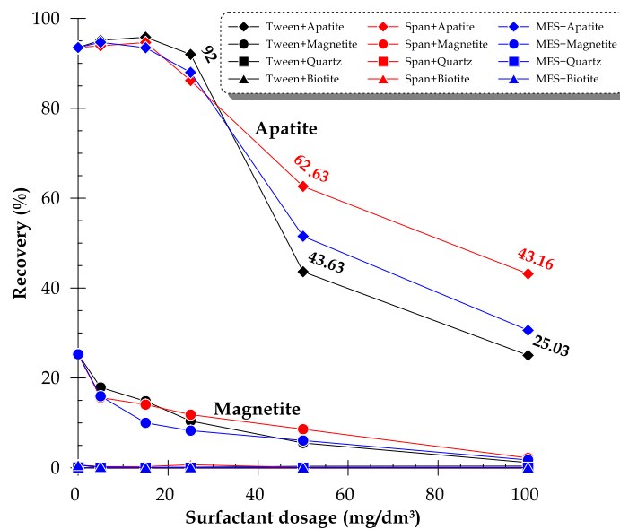
Fig. 5. The effect of the surfactant dosage on the single minerals flotation (Pulp density: 10%, fatty acid dosage: 200 mg/dm 3 , pH 8.0, temperature: 25°C, flotation time: 3 min, and surfactant dosage: 0-100 mg/dm 3 )
