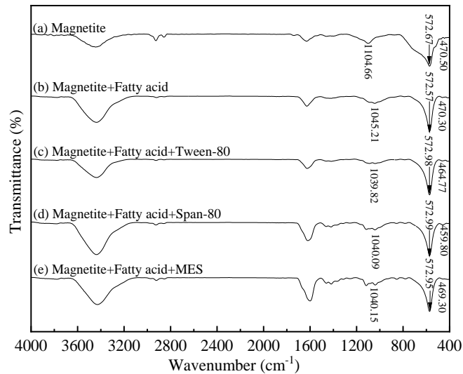
Fig. 9. FTIR spectra of magnetite treated by the reagents at pH 8 and 25^{\circ}\text{C} (Fatty acid dosage: 200\text{ mg/dm}^3 , surfactant dosage: 15\text{ mg/dm}^3 )
