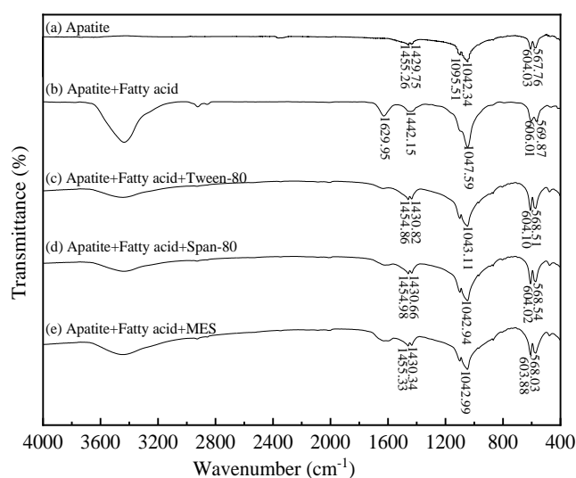
Fig. 8. FTIR spectra of apatite treated by the reagents at pH 8 and 25°C (Fatty acid dosage: 200 \text{mg}/\text{dm}^3 , surfactant dosage: 15 \text{mg}/\text{dm}^3 )
