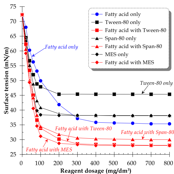
Fig. 6. The surface tension of the tested solution with various reagents and concentrations (Fatty acid dosage: 200 mg/dm 3 , surfactant dosage: 15 mg/dm 3 , temperature: 25°C, and pH 8.0)
