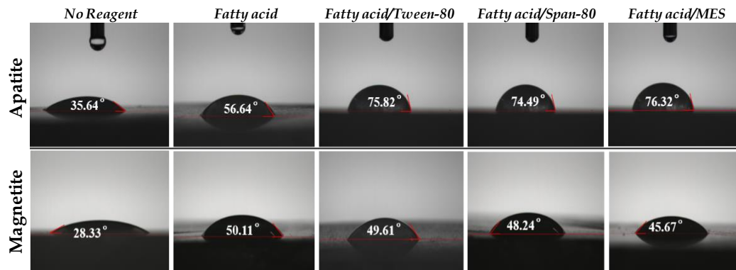
Fig. 10. The contact angle of the minerals before and after treated with reagents (Fatty acid dosage: 200 mg/dm 3 , surfactant dosage: 15 mg/dm 3 )
