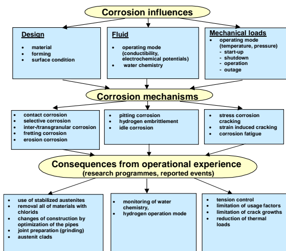
Figure 6. Root causes of different corrosion mechanisms and the operational implementation of protection goals in nuclear power plants
