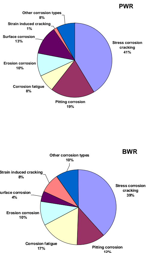
Figure 5. Distribution of corrosion types in PWR and BWR plants in Germany (Evaluation of reportable events 1968 – 2001).
