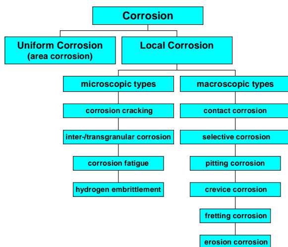
Figure 2. Outline of corrosion types
