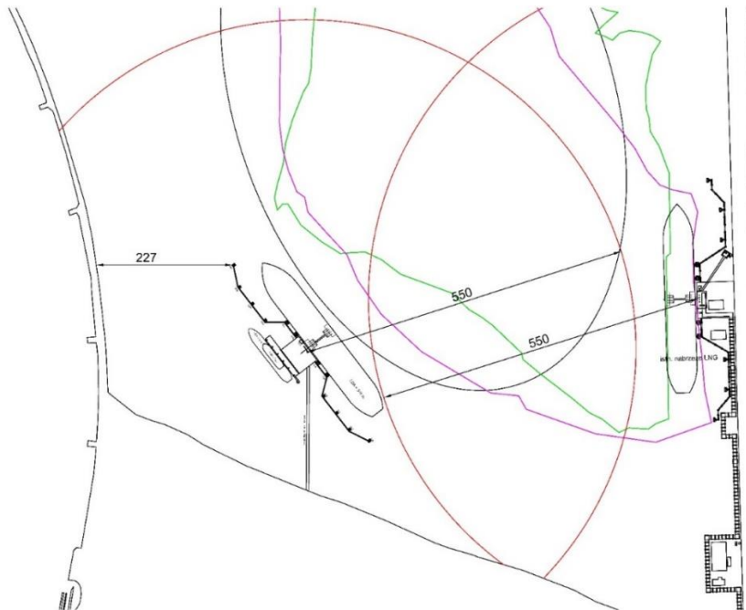
Fig. 2. Preliminary location of the universal LNG transshipment facility and the existing LNG discharge berth
