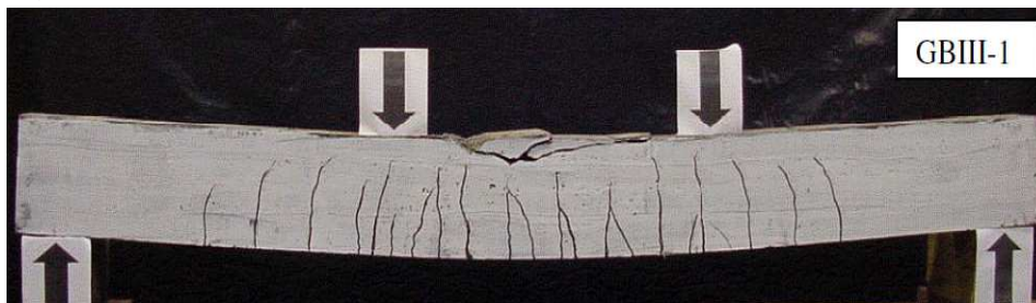
Fig. 10. Example of reinforced concrete beams from geopolymeric concrete damage [28]
