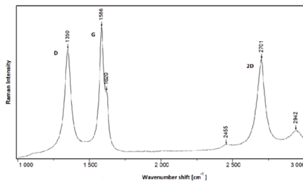
Figure 2. Raman spectrum of graphene flakes
