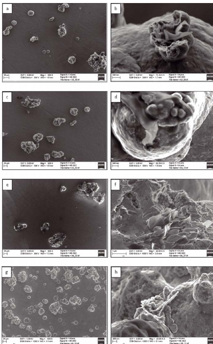
Figure 4. Surfaces of Ni/graphene composite coatings on different rows samples with different amount of graphene are presented in \text{g}/\text{dm}^3 : a, b): 0.1; c, d): 0.2; e, f): 0.5; g, h): 1.0; on the left column (a, c, e, g) low magnification images, on the right column (b, d, f, h) high magnification images
