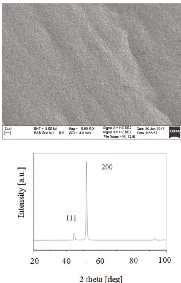
Figure 3. Images of surface and diffraction pattern of the Ni coating
