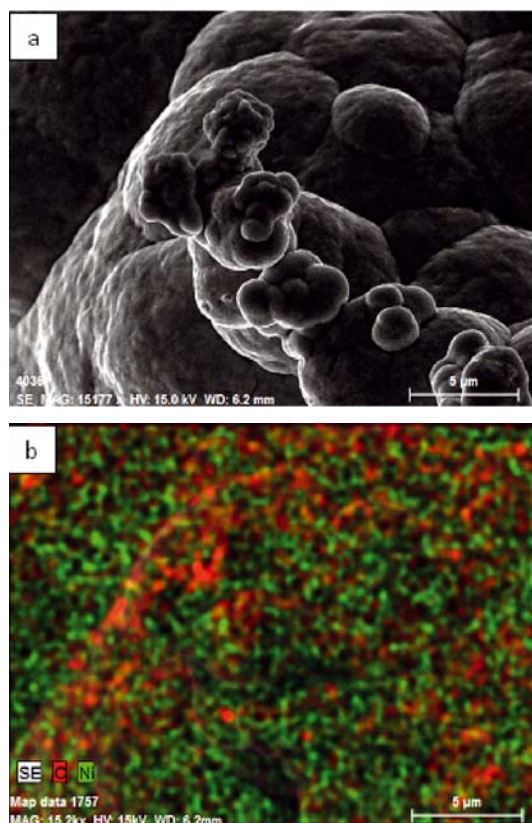
Figure 5. EDS analysis of chemical composition of Ni/graphene coating material (0.5 g/dm 3 ), a) surface of the coating; b) map of the elements (red – C, green - Ni)
