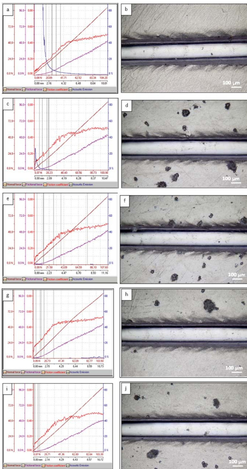
Figure 8. Diagram showing change of parameters during scratch-test process and image of scratch of the coatings: a, b) Ni; c, d) 0.1 g/dm 3 ; e, f) 0.2 g/dm 3 ; g, h) 0.5 g/dm 3 ; i, j) 1.0 g/dm 3
