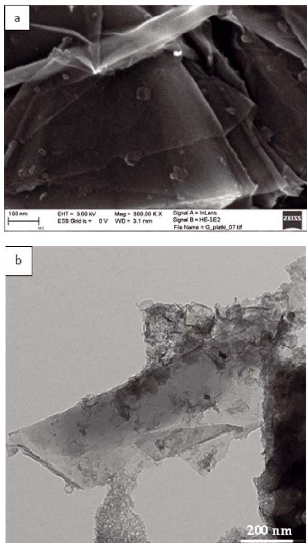
Figure 1. SEM (a) and TEM (b) images of graphene flakes
