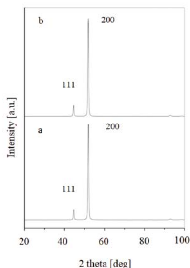
Figure 6. Diffraction pattern of Ni/graphene composite coatings: a) 0.2 g/dm 3 ; b) 1.0 g/dm 3
