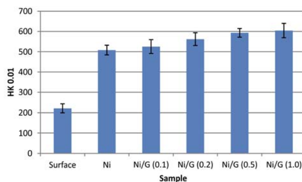
Figure 7. Microhardness of substrate material, Ni coating and Ni/G composite coatings
