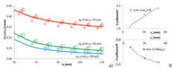
Fig. 7 External bar model. FEM results and fitting curves related to b_e and c_c
