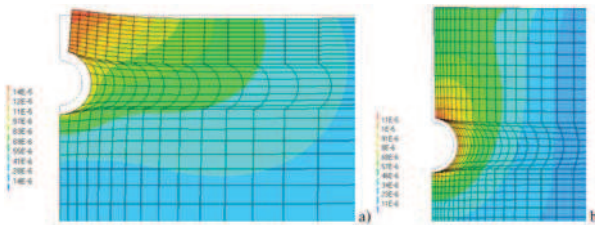
Fig. 2 FEM deformed shape: a) c_c = 10 \text{ mm} - R_0 = 5 \text{ mm} - b_i = 125 \text{ mm} , b) c_c = 50 \text{ mm} - R_0 = 10 \text{ mm} - b_i = 80 \text{ mm}
