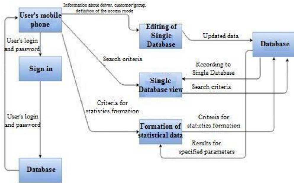
Fig. 3. Model of the subsystem "Single order database and travel control control" for the user with the role of Administrator.
