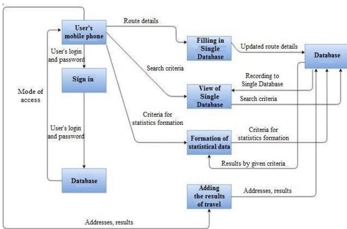
Fig.4. Model of the subsystem "Single order database and trip control" for the user with the role of driver.
