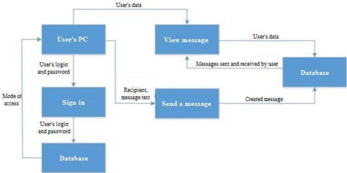
Fig. 6. Modular structure of the subsystem "Messaging".
