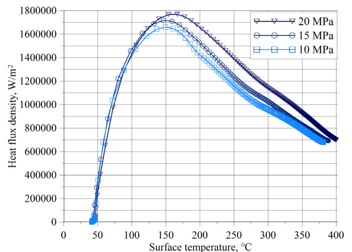
Fig. 4. The value of heat flux density as a function of surface temperature for different pressure forces
