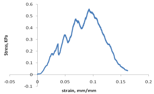
Fig. 3. Stress-strain curve at 22% clay content
