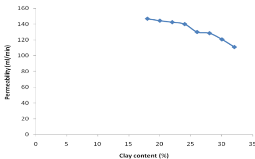
Fig. 11. Variation of clay content and permeability
