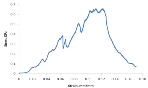
Fig. 4. Stress-strain curve at 26% clay content
