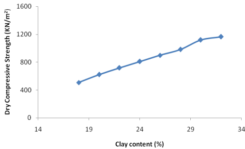
Fig. 10. Variation of clay content and dry compressive strength
