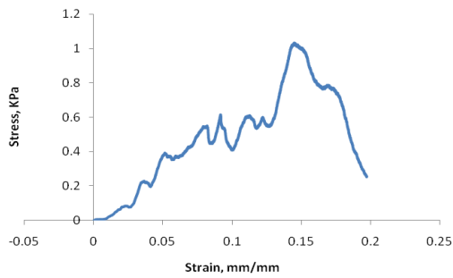
Fig. 6. Stress-strain curve at 32% clay content
