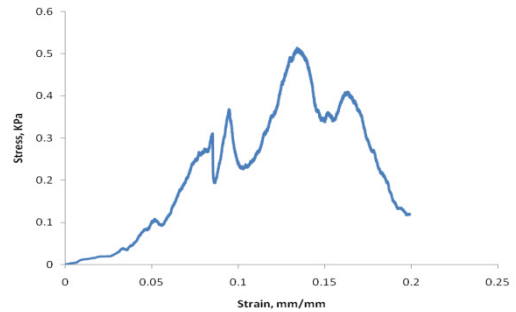
Fig. 2. Stress-strain curve at 18% clay content
