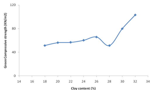
Fig. 9. Variation of clay content and Green compressive strength
