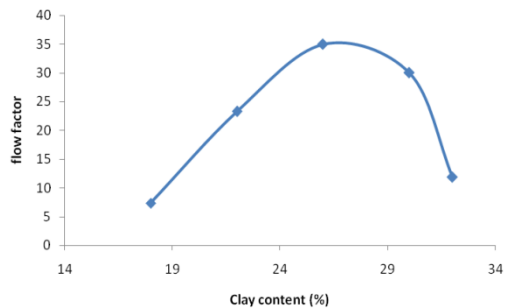
Fig. 7. Variation of clay content and flowability for set point 85% and 50%
