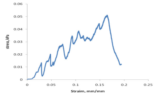
Fig. 5. Stress-strain curve at 30% clay content
