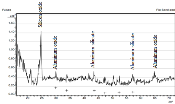
Fig. 1. XRD of the Isasa River Sand
