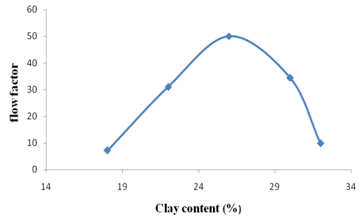
Fig. 8. Variation of clay content and flowability for set point 85% and 60%
