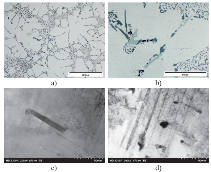
Fig. 1. Microstructure of AlSi7Mg alloy in the as-cast condition; a, b) LM; c, d) STEM.
