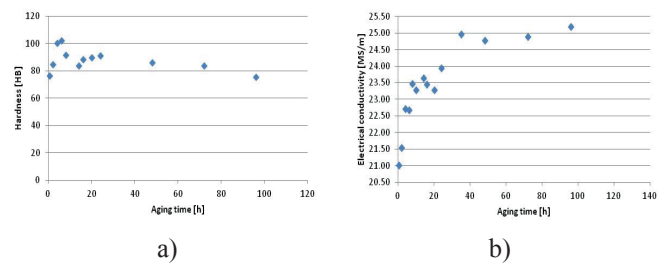
Fig. 10. AlSi7Mg alloy properties after aging at 180°C for different times; a) Hardness; b) Electrical conductivity.
