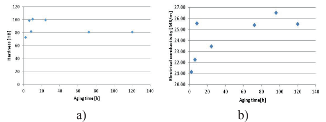
Fig. 11. Solutioned for 48h AlSi7Mg alloy properties after aging at 180°C for different times; a) Hardness; b) Electrical conductivity.
