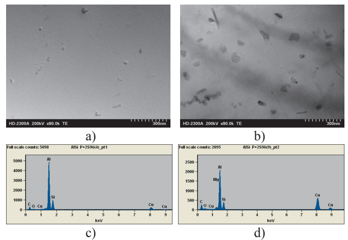
Fig. 6. Equiaxed phases within the \alpha-Al dendrites, STEM; a) after 6h of aging at 180^\circ C ; b) after 94h of aging at 180^\circ C ; c, d) EDS spectra from these phases (Cu from the handle).
