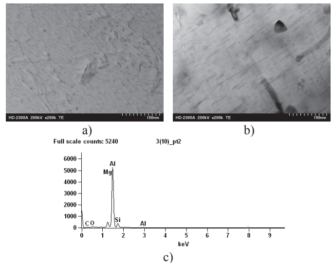
Fig 5. Fine needle- or plate-like precipitates within the \alpha-Al dendrites, STEM; a) after 6h of aging at 180^\circ C ; b) after 94h of aging at 180^\circ C ; c) EDS spectrum from these phases.
