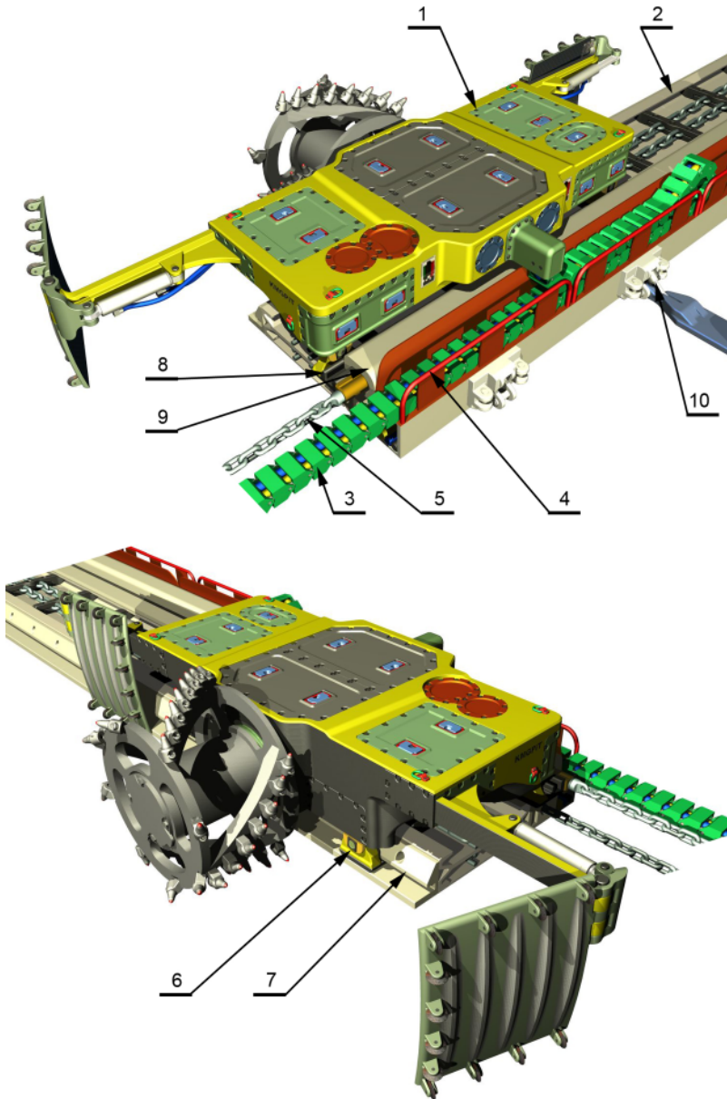
Fig. 9. Single cutting head shearer moving on the conveyor (Boloz, 2012)
