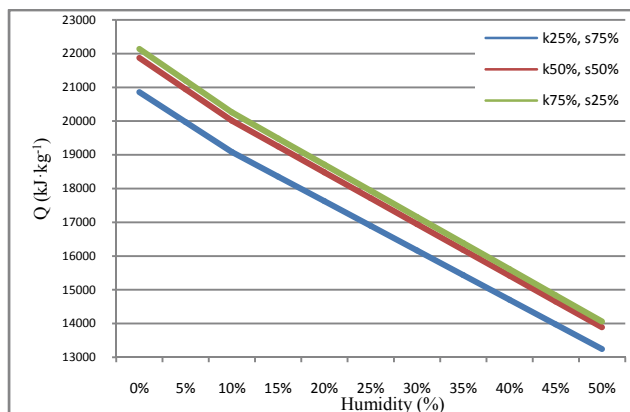
Figure 3. Calorific value of the mixtures of coffee grounds and wheat straw depending on their moisture
