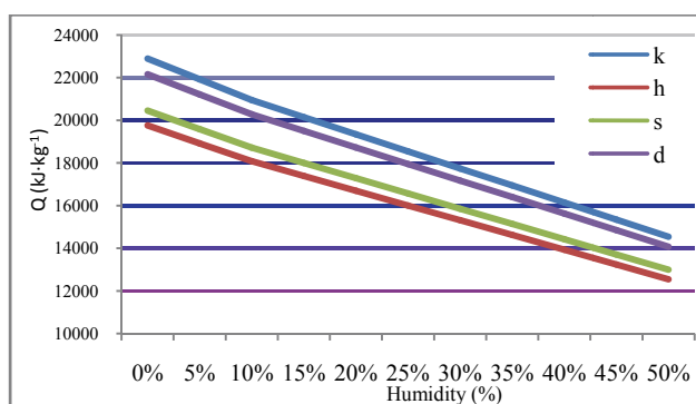
Figure 1. The calorific value of uniform substrates
