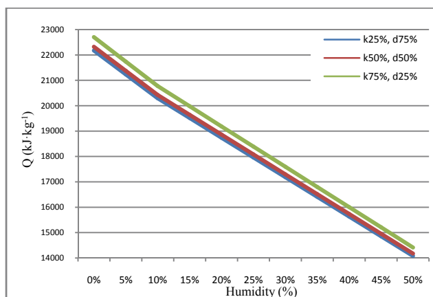
Figure 4. Calorific value of the mixtures of coffee grounds and pine wood depending on their moisture
