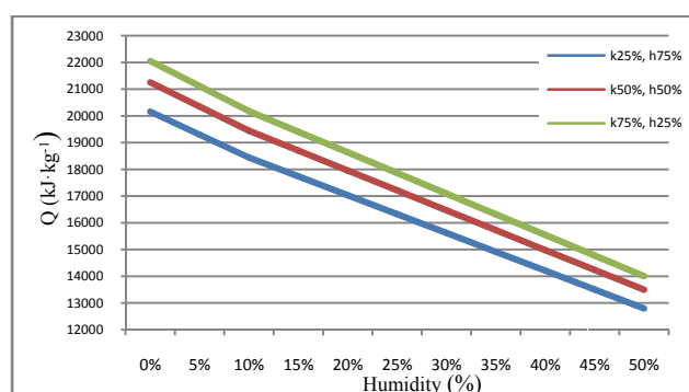
Figure 2. Calorific value of the mixtures of coffee and tea grounds depending on their moisture
