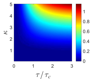
Fig. 3. The normalized decrement \chi(\kappa, \tau)/\chi(1, \tau_c) shown as a function of delay time \tau and normalized wave number \kappa .
