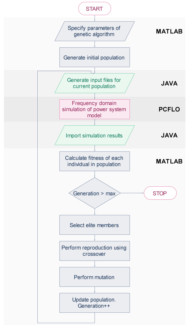
Fig. 5. Block diagram of the developed algorithm of optimum APF allocation
