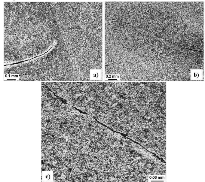
Fig. 3. Microstructure of FSW lap joint of aluminium alloy 6082; a) „hooking” of material; b) effective sheet thickness reduction; c) „kissing bond” ( Al_2O_3 inclusions)
