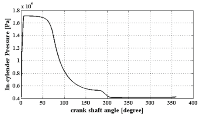
Figure 5. Variations of in-cylinder pressure against crank angle at ω = 1000 rpm
