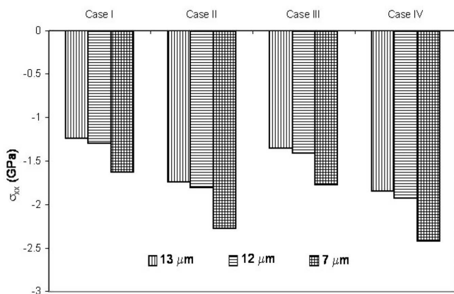
Fig. 10. Stress distribution on the outer boundary of MgO-ZrO 2 coating for different cases
