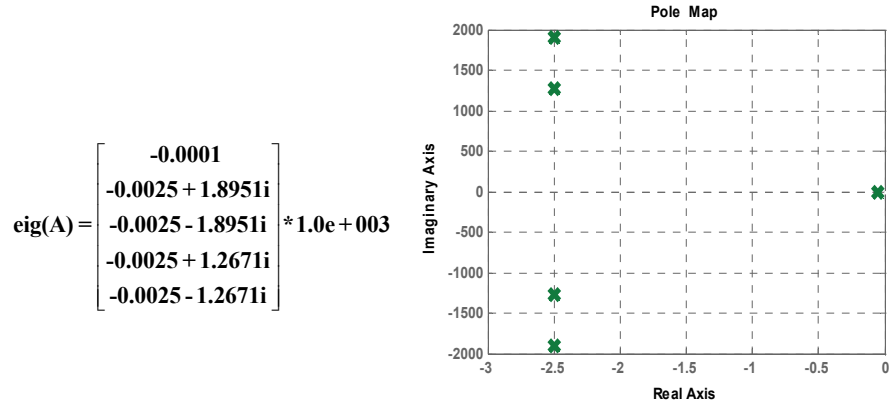
Fig. 2. Poles (x) plotting for the system stability
