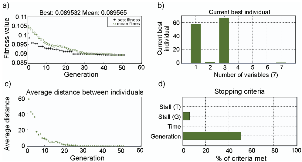
Fig. 11. (a) Best & mean values at every generation, (b) Final 7 best individual values which minimize the cost function, (c) Average Distance between Individuals vs. Number of Generations, (d) Stopping Criterion for the Genetic Optimization
