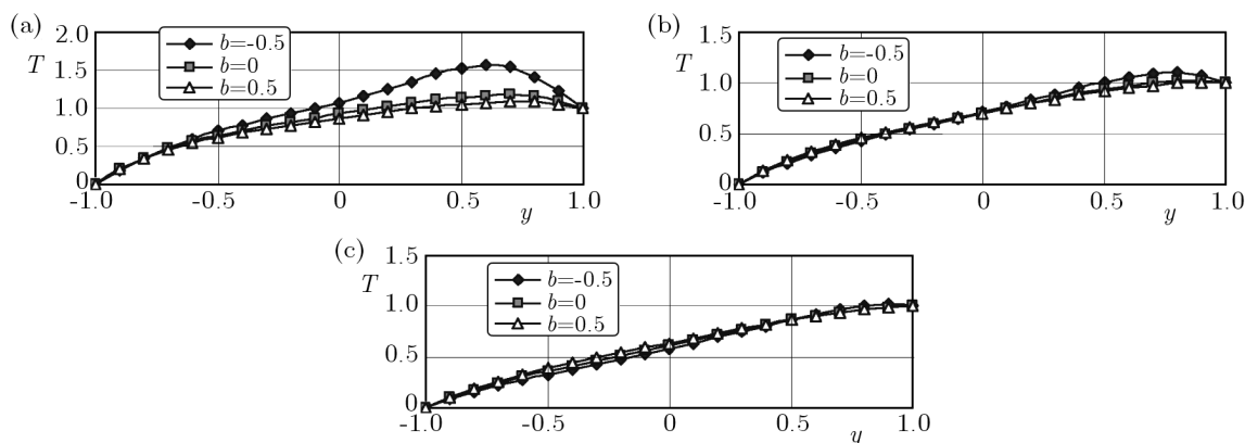
Fig. 3. Variation of T with y for various values of b ; (a) a = 0 , M = 0 , (b) a = 0 , M = 1 , (c) a = 0 , M = 2
