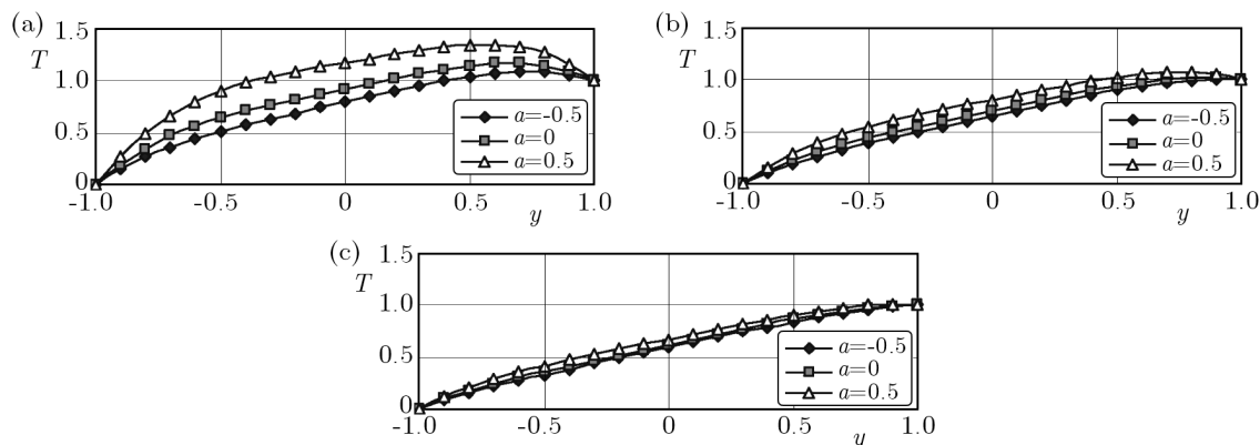
Fig. 2. Variation of T with y for various values of a ; (a) b = 0 , M = 0 , (b) b = 0 , M = 1 , (c) b = 0 , M = 2
