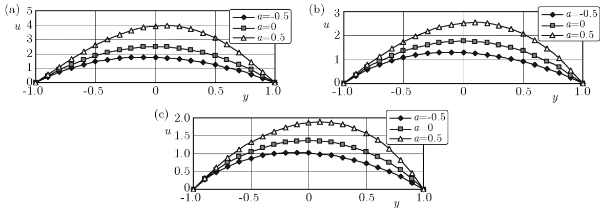
Fig. 1. Variation of u with y for various values of a ; (a) b = 0 , M = 0 , (b) b = 0 , M = 1 , (c) b = 0 , M = 2
