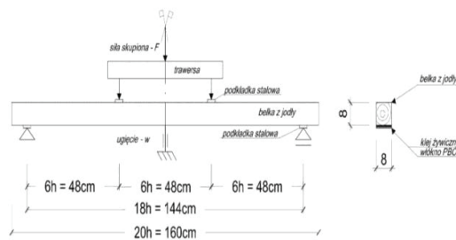
Fig. 1. Static diagram of the system for determining the modulus of elasticity of the tested wood
