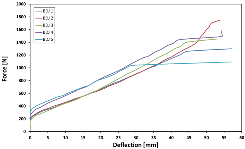
Fig. 5. Graph of dependence "load - deflection" for the tested elements of BDJW
