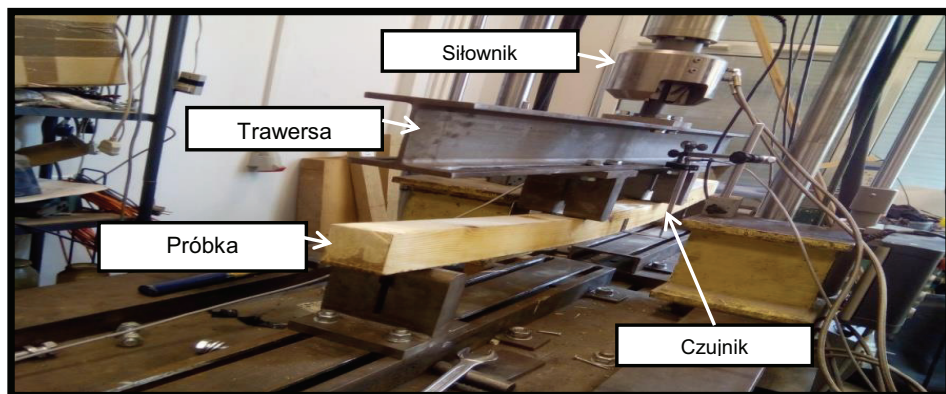
Fig. 2. Test stand for static loads
