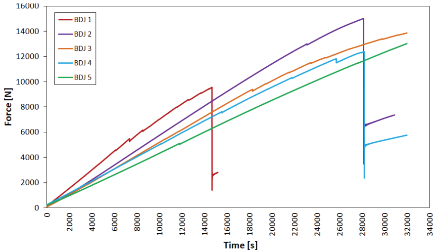
Fig. 4. Diagram of the " load - time" relationship for the tested BDJ elements
