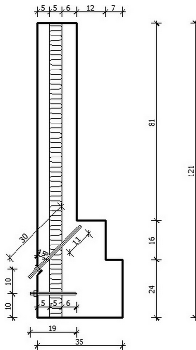
Figure 13. Distribution diagram of COPY-ECO anchors.
