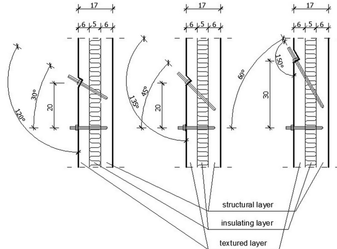
Figure 18. Alternative to two-anchor systems, inverted systems.
