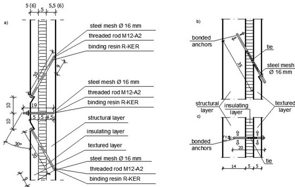
Figure 12. Wiring diagram with steel ties: a) solutions for staircase walls, b) solutions for gable wall panels.
