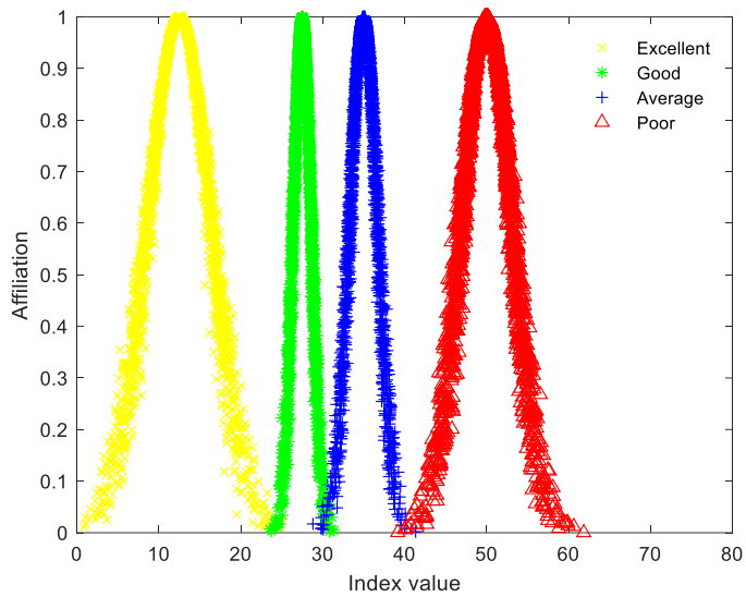
Fig. 4. Cloud drop diagram of average travel time consumption of passengers
