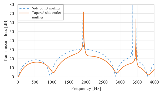
Fig. 6. Comparison of FEA of side outlet muffler and tapered side outlet muffler.
