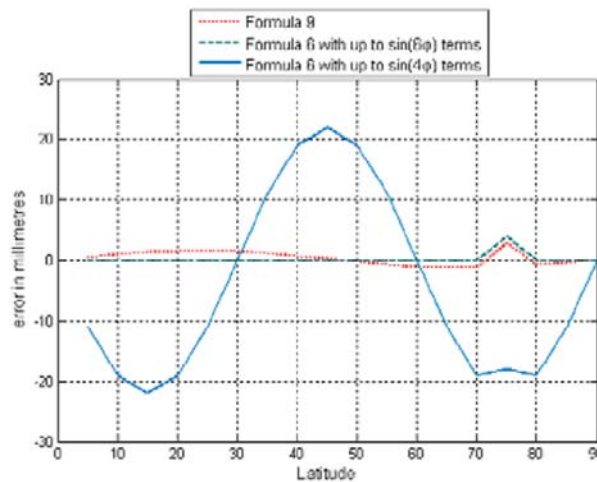
Fig. 2. Error assessment of formulas providing submeter accuracies [9]
