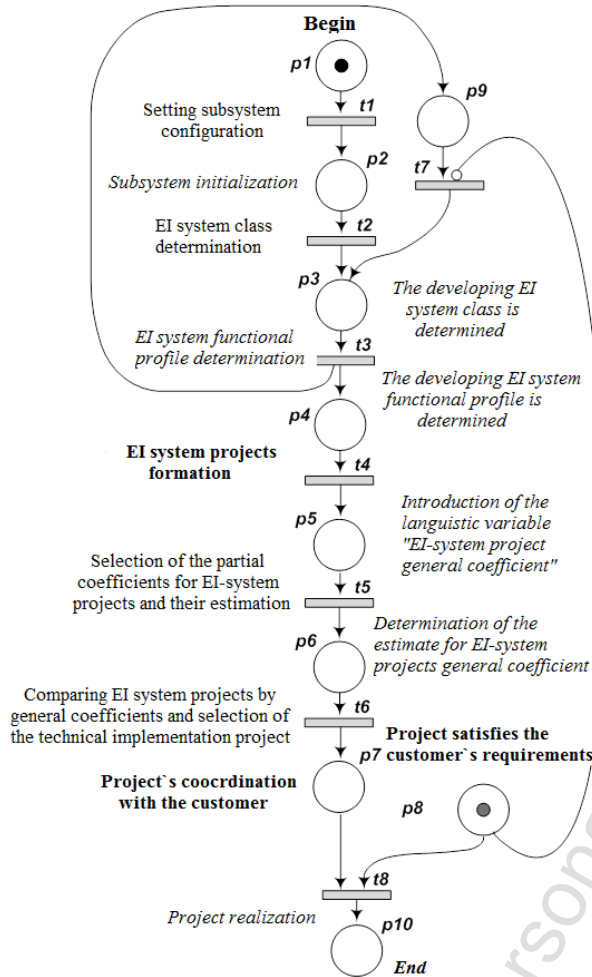
Fig. 1. The developed model based on Petri nets
