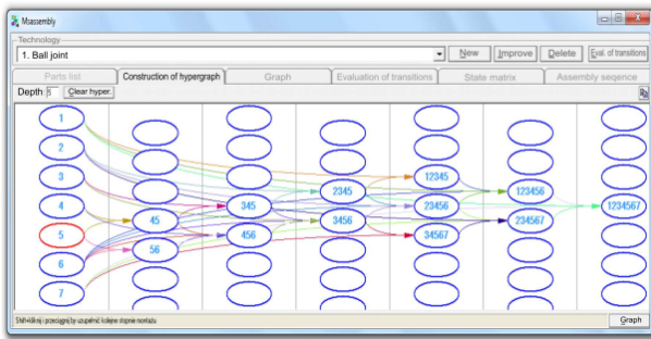
Fig. 6. Directed hypergraph of the construction structure for a ball joint (Msassembly program).
