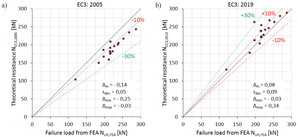
Fig. 7. Comparison of theoretical block tearing resistance with ultimate resistance obtained from numerical simulations N_{ult,FEA} : a) for current Eurocode 3 [3], b) for new proposal [4]
