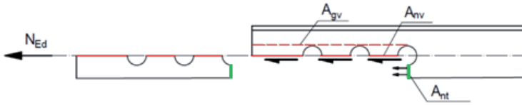
Fig. 1. Schema of block tearing in steel angle member connected by one leg
