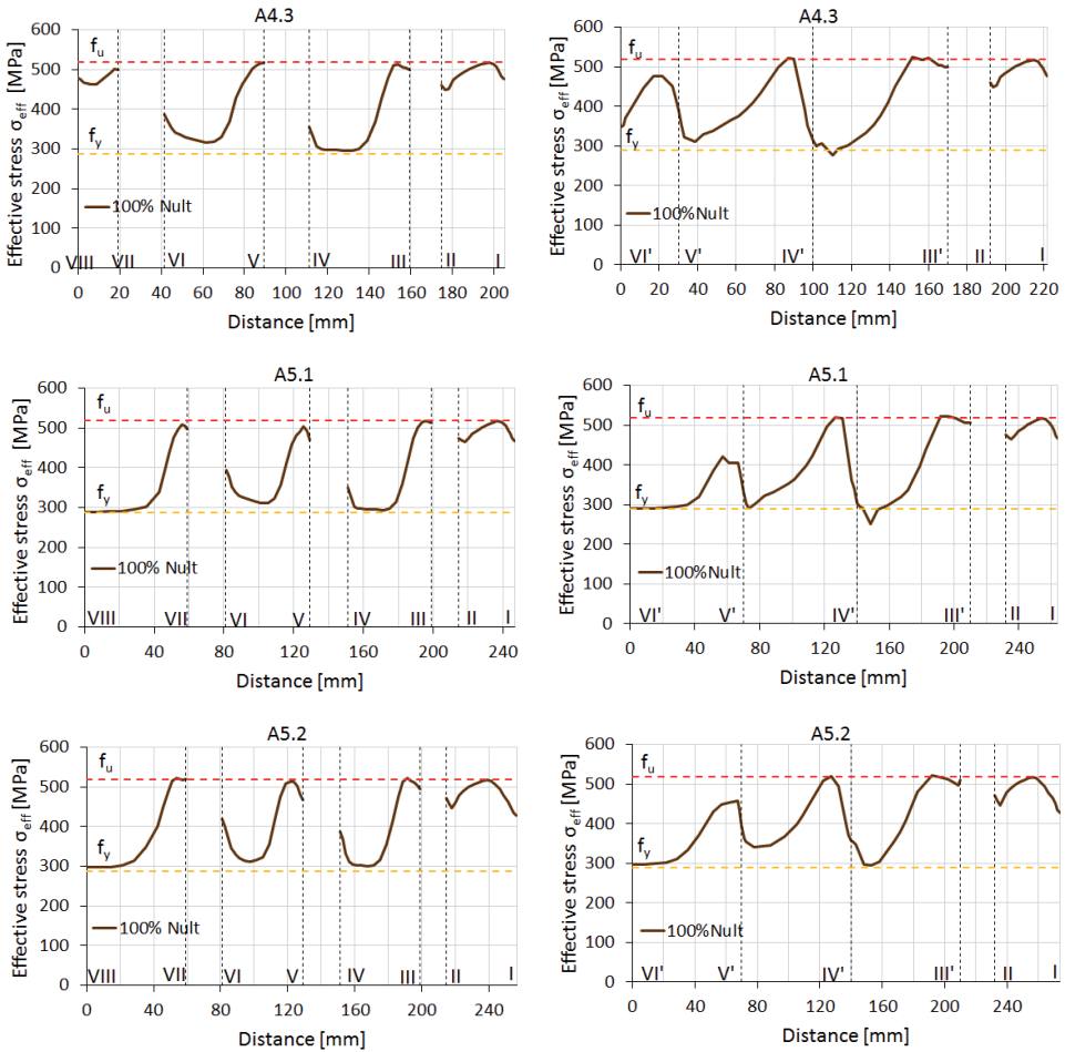
Fig. 6. Distribution of effective stresses \sigma_{eff} for the failure load N_{ult,FEA} (left diagram shows distribution along net tension and net shear area; right one shows distribution along net tension and gross shear area)
