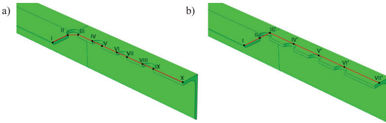
Fig. 5. Paths definitions in which distribution of stresses were observed: a) in net area subjected to shear, b) in gross area subjected to shear
