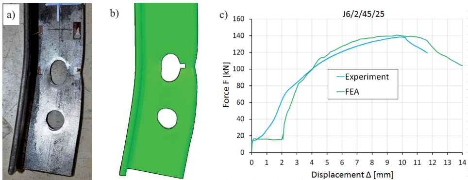
Fig. 3. Specimen J6/2/45/25: a) failure initiation obtained in the experimental test, b) visible symptom of fracture initiation in FE model, c) comparison of obtained force-displacement curves.
