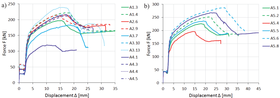
Fig. 4. Force-displacement curves: a) for equal leg angles, b) for unequal leg angles
