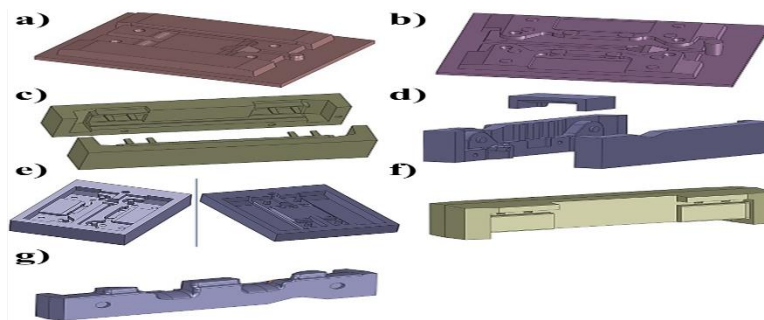
Fig. 4. a) bottom plate; b) top plate; c) large core box; d) small core box; e) casting mold halves; f) large core; g) small core
