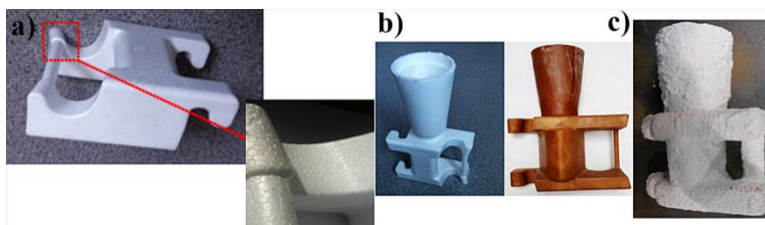
Fig. 8. a) model foamed in a metal die; b) models with a gating system: polystyrene and wax; c) shell mold
