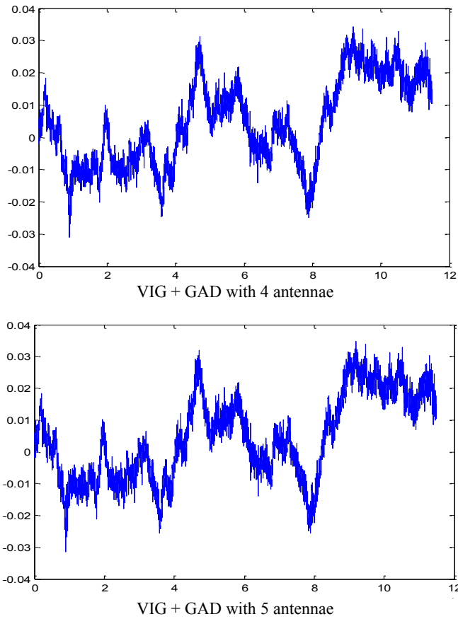
Fig. 10. Roll ( \phi ) error time histories [own study]
