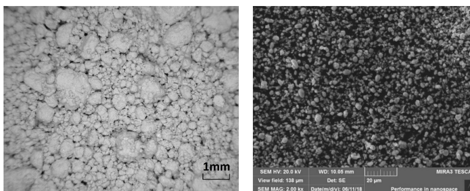
Fig. 1. Optical observation of tin sludge
