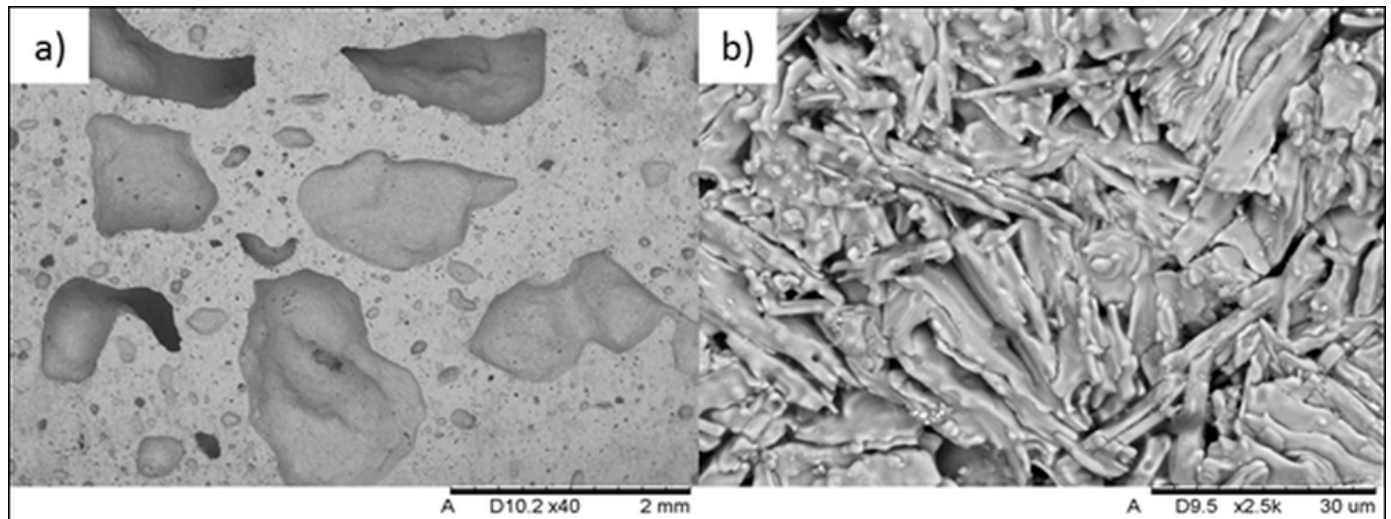
Fig. 1. Manufactured MAX phase preform: a) view of the overall open porosity, b) microstructure of MAX phase platelets
