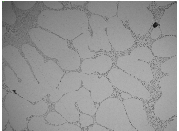
Fig. 17. Microstructure of the sample cast without applying pressure, zoom 400x, etching 0.5% HF
