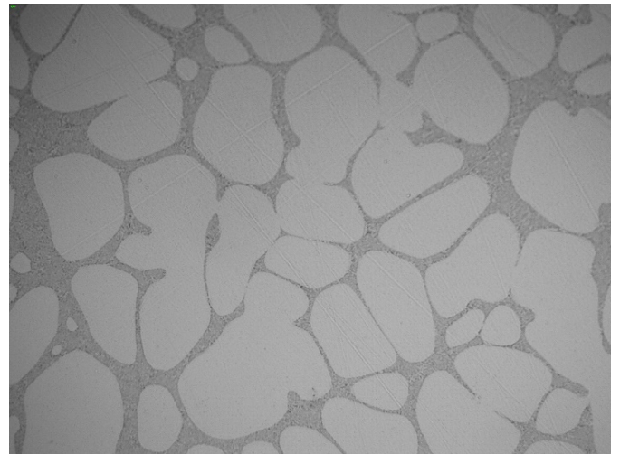
Fig. 19. Microstructure of the sample cast under pressure with value 150 MPa, zoom 400x, etching 0.5% HF
