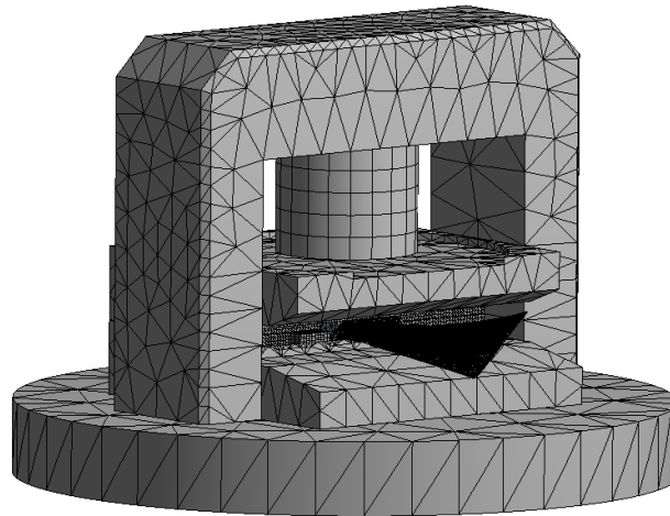
Fig. 1. Blade holder discrete model
