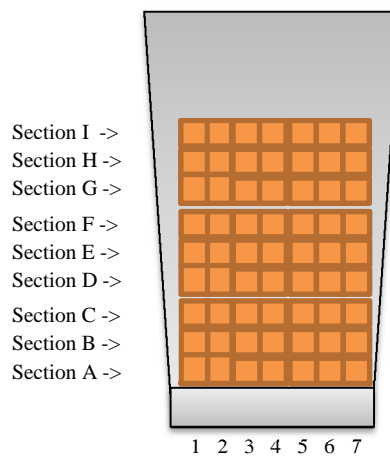
Fig. 6. Strain gauges joint location on blade surface
