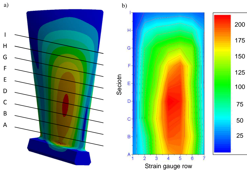
Fig. 10. Blade strain distribution comparison of a) numerical and b) experimental methods
