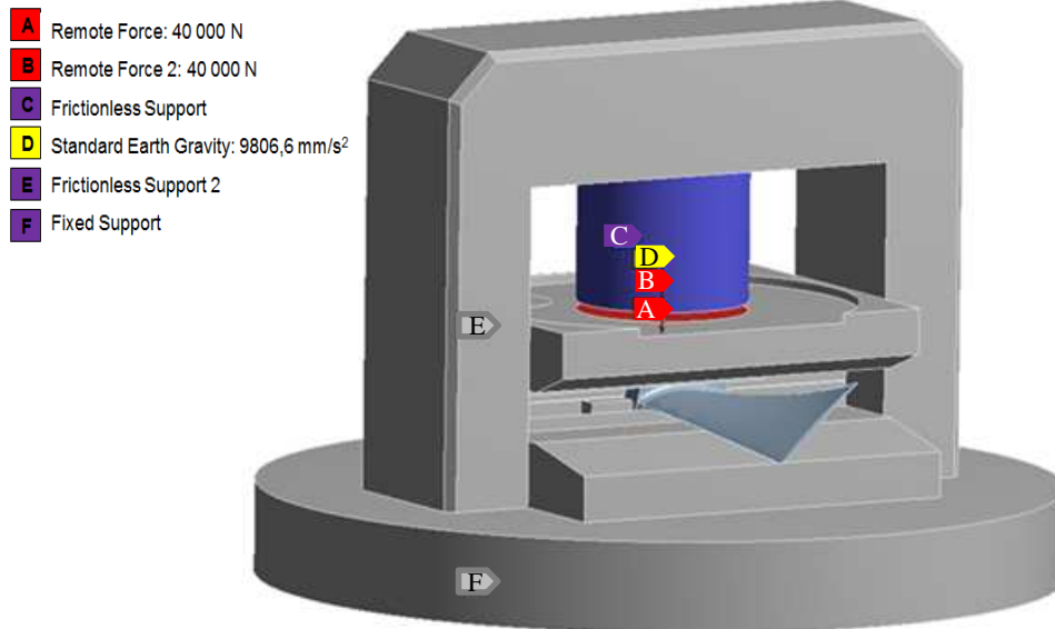
Fig. 3. Holder model with boundary conditions
