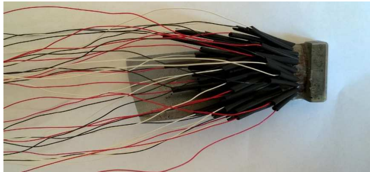
Fig. 7. Instrumented blade for deformation distribution measurement
