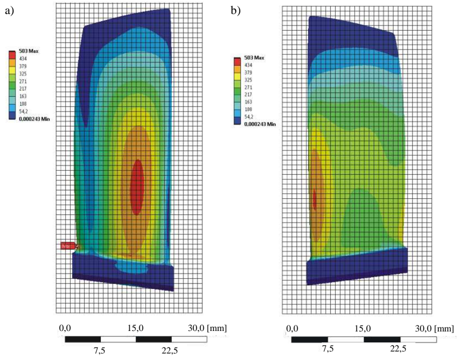
Fig. 9. Blade strain distribution on a) suction and b) pressure side
