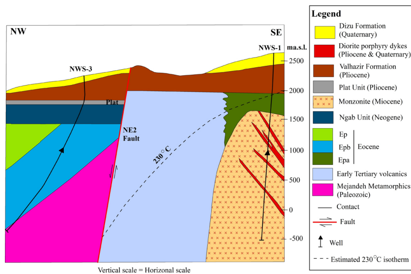
Fig. 3. Schematic transverse section of the study area and position, depth and formation of the exploration wells in the Moyil Valley
