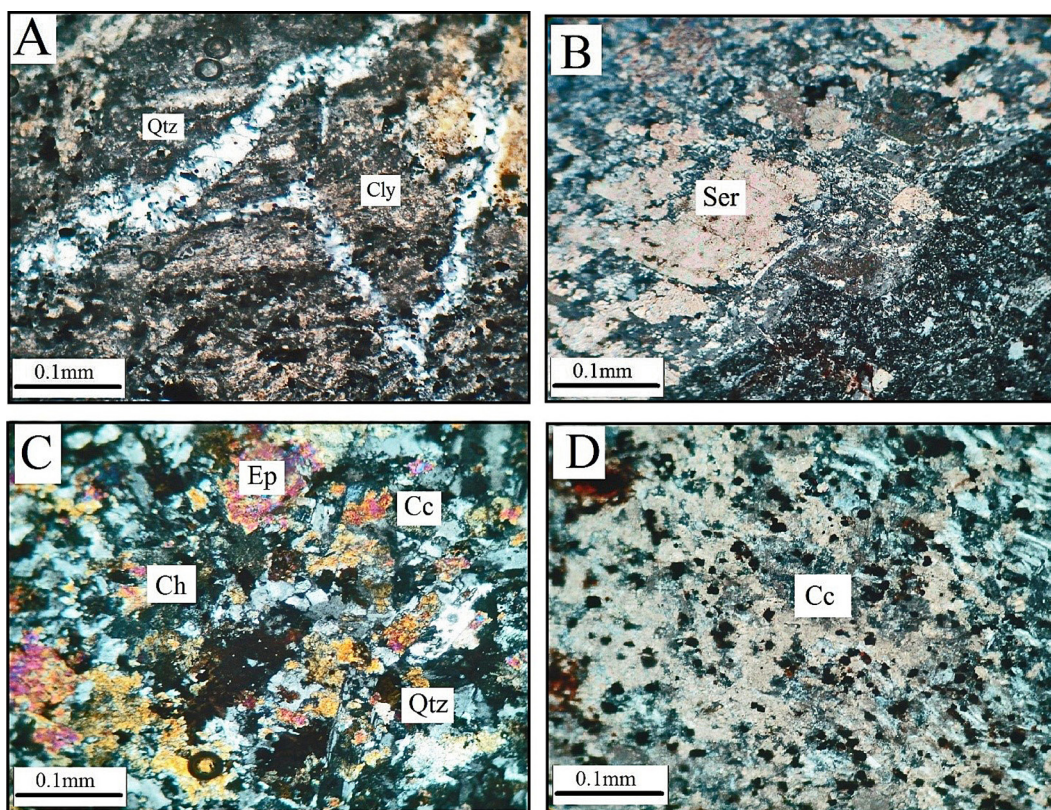
Fig. 4. Microscopic images of material from well NWS-3. A - Argillic alteration of clay minerals (Cly) and quartz veinlets (Qtz); B - Sericite (Ser) in the phyllic alteration zone; C - Epidote (Ep), chlorite (Ch) and calcite (Cc) in the propylitic alteration zone; D - Calcite (Cc) in the calcitic alteration zone
