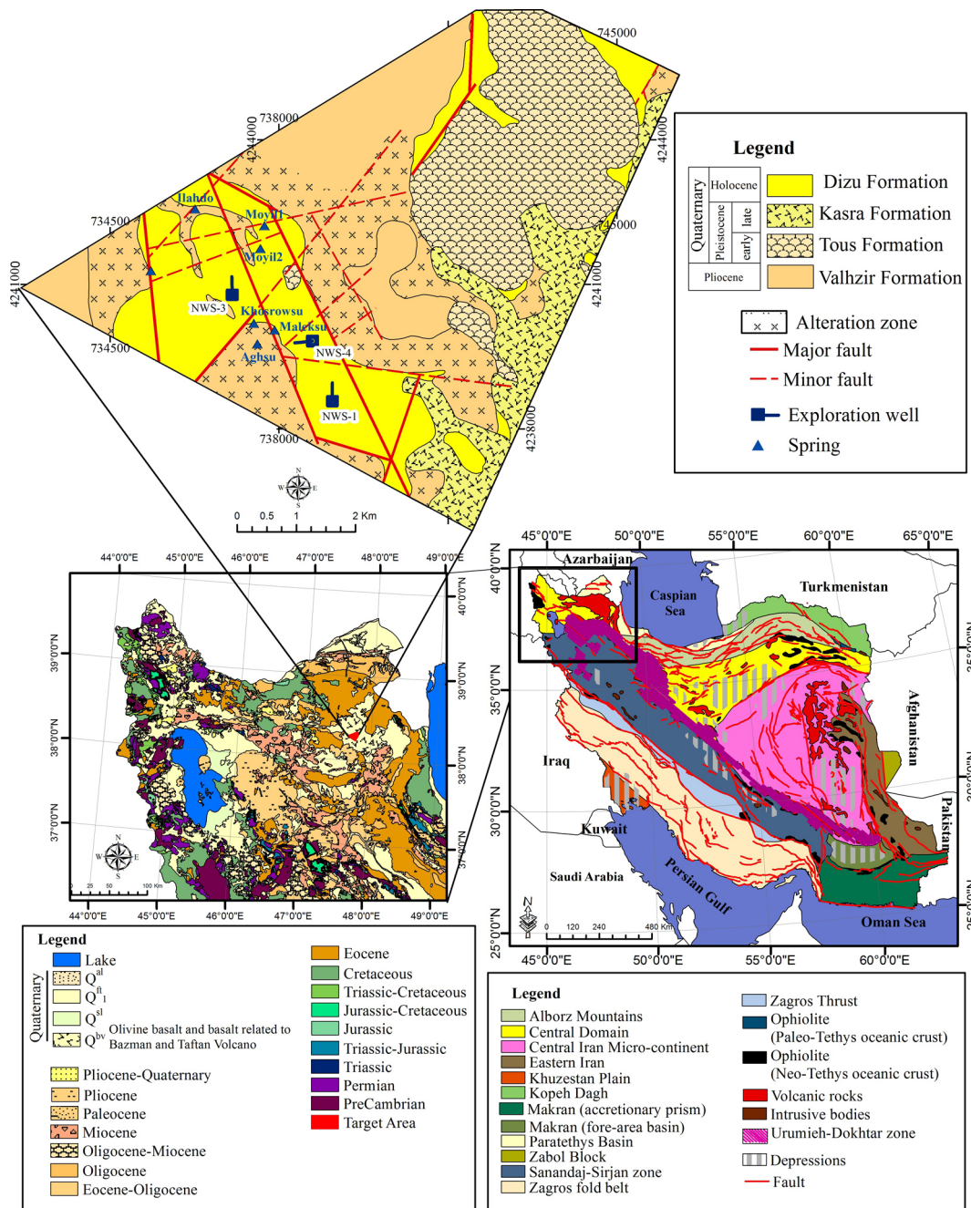
Fig. 2. Location of the study area (northwest Iran), with a simplified map of the different formations to the northwest of Mountain Sabalan (modified from Bogie et al., 2000)
