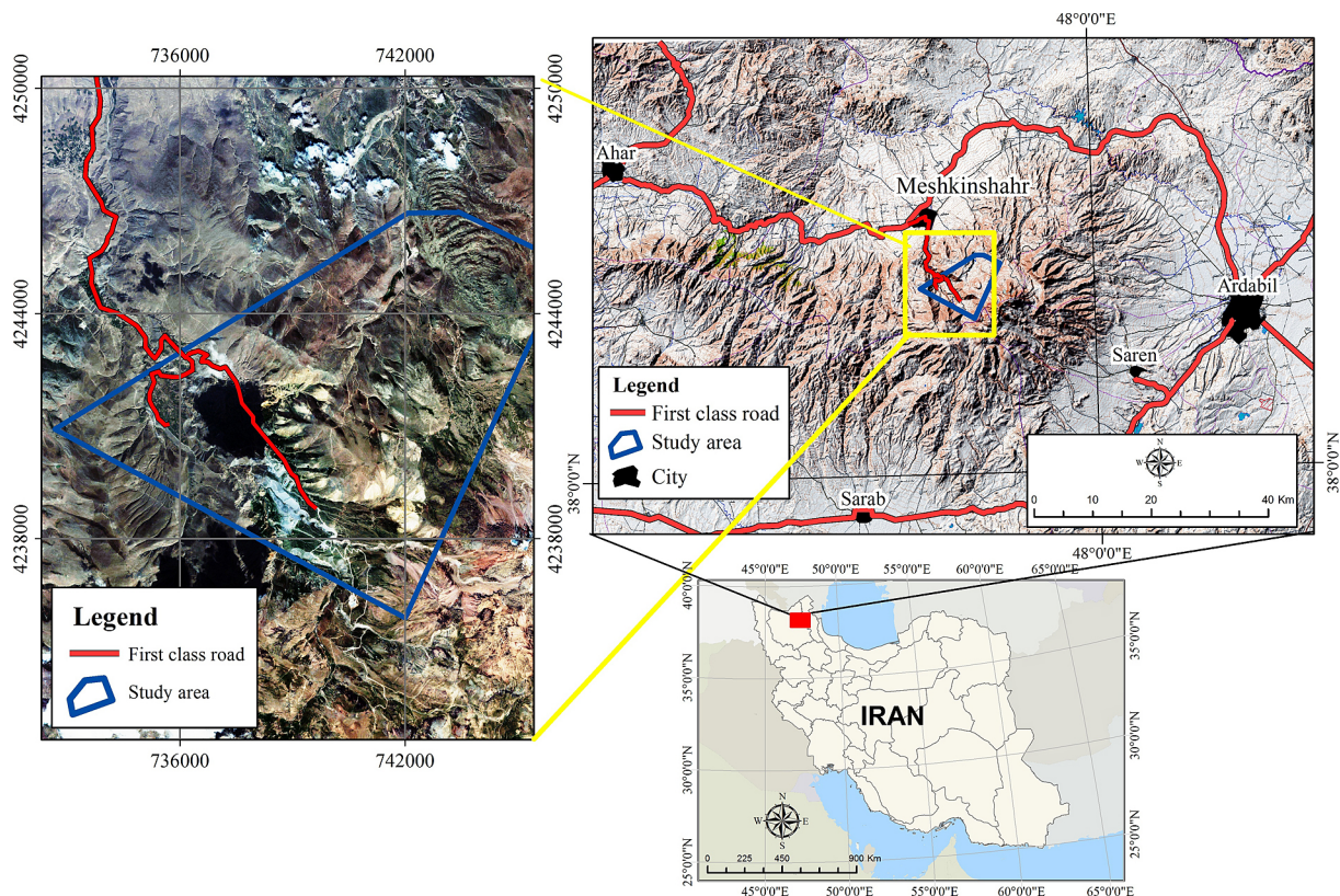
Fig. 1. Location of the Moyil Valley in northwest Iran
