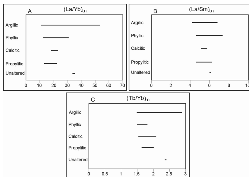
Fig. 6. Comparison of trends in changes in values of: A - (La/Yb)_{cn} ; B - (La/Sm)_{cn} ; C - (Tb/Yb)_{cn} for argillic, phyllic, propylitic and calcitic alterations with trachyandesite
