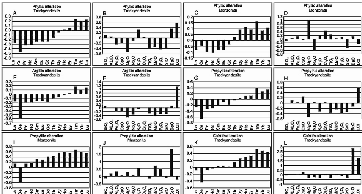
Fig. 5. Histogram corresponding to an increase or decrease in the mass of main elements and REEs hydrothermal alteration zones related to trachyandesite and monzonite rock unit. A, B - REEs and basic elements of the phyllic alteration zone in trachyandesite; C, D - REEs and main elements of the phyllic alteration zone in monzonite; E, F - REEs and main elements of the argillic alteration zone in trachyandesite; G, H - REEs and basic elements of the propylitic alteration zone in trachyandesite; I, J - REEs and main elements of the propylitic alteration zone in monzonite; K, L - REEs and main elements of the calcitic alteration zone in trachyandesite
