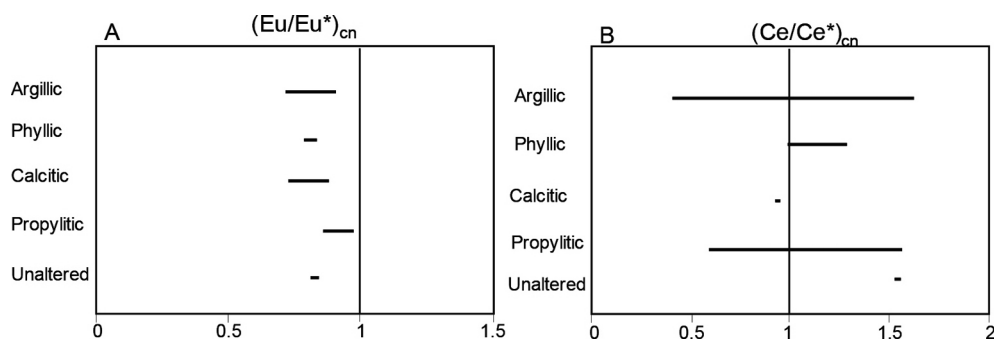
Fig. 7. Comparison of trends in changes in values of: A - (Eu/Eu^*)_{cn} ; B - (Ce/Ce^*)_{cn} for argillic, phyllic, propylitic and calcitic alterations with trachyandesite
