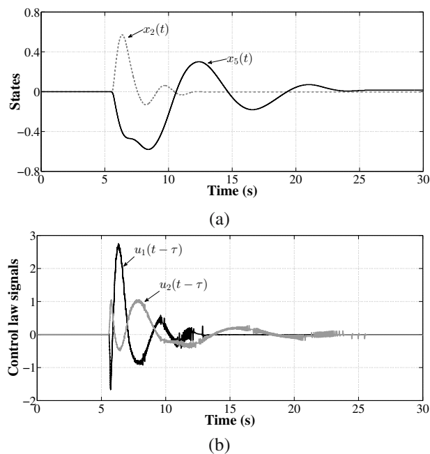
Fig. 2. State evolution of the TRMS under the control law (6) obtained via Theorem 3 with \tau = 0.27 , \sigma = 0.25 (a). Time evolution of the control signals (b).
