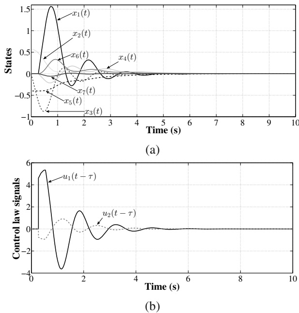
Fig. 1. State evolution of the TRMS under the control law (6) obtained via Theorem 3 with \tau = 0.27 , \sigma = 0.25 (a). Time evolution of the control signals (b).
