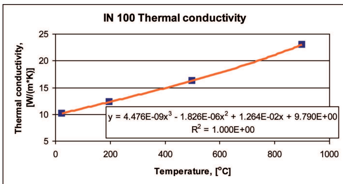
Fig. 2. Thermal conductivity of IN 100 alloy vs. temperature
