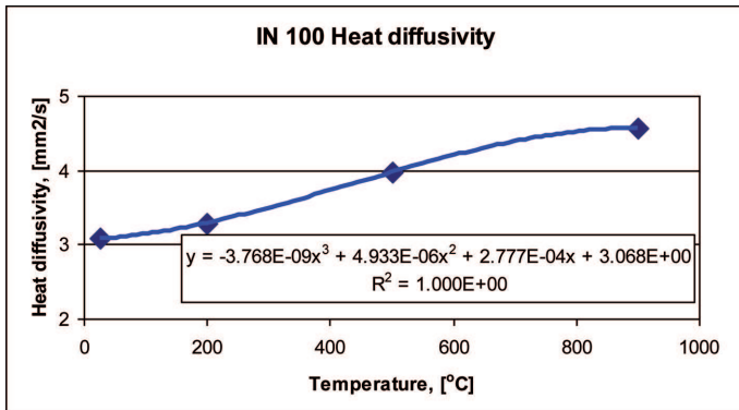
Fig. 1. Heat diffusivity of IN 100 alloy vs. temperature
