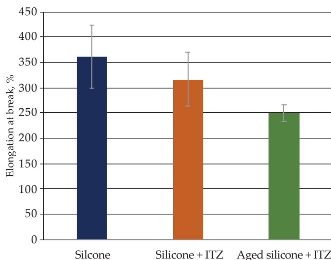
Fig. 6. Elongation at break for reference material, the unaged and aged drug-silicone composite
