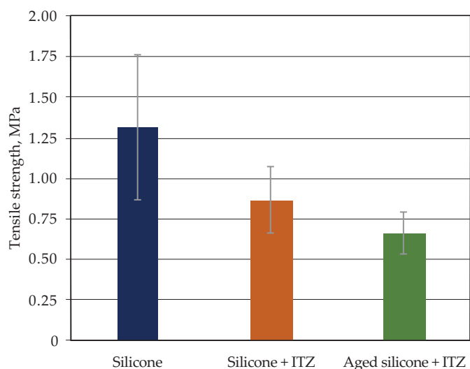
Fig. 5. Tensile strength for reference material, the unaged and aged drug-silicone composite
