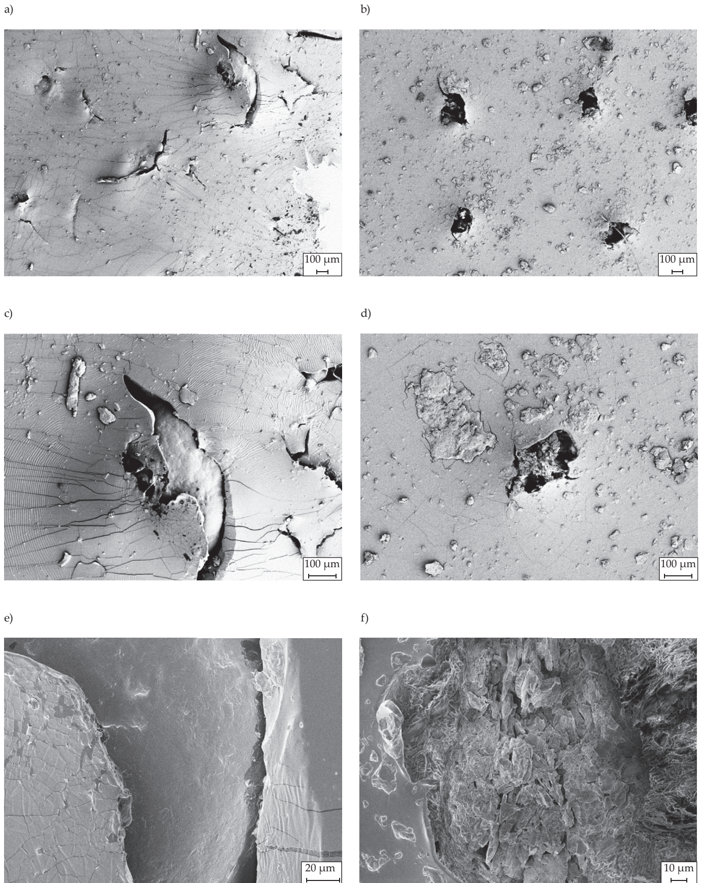
Fig. 7. SEM micrographs of native (a, c, e) and aged samples (b, d, f)
