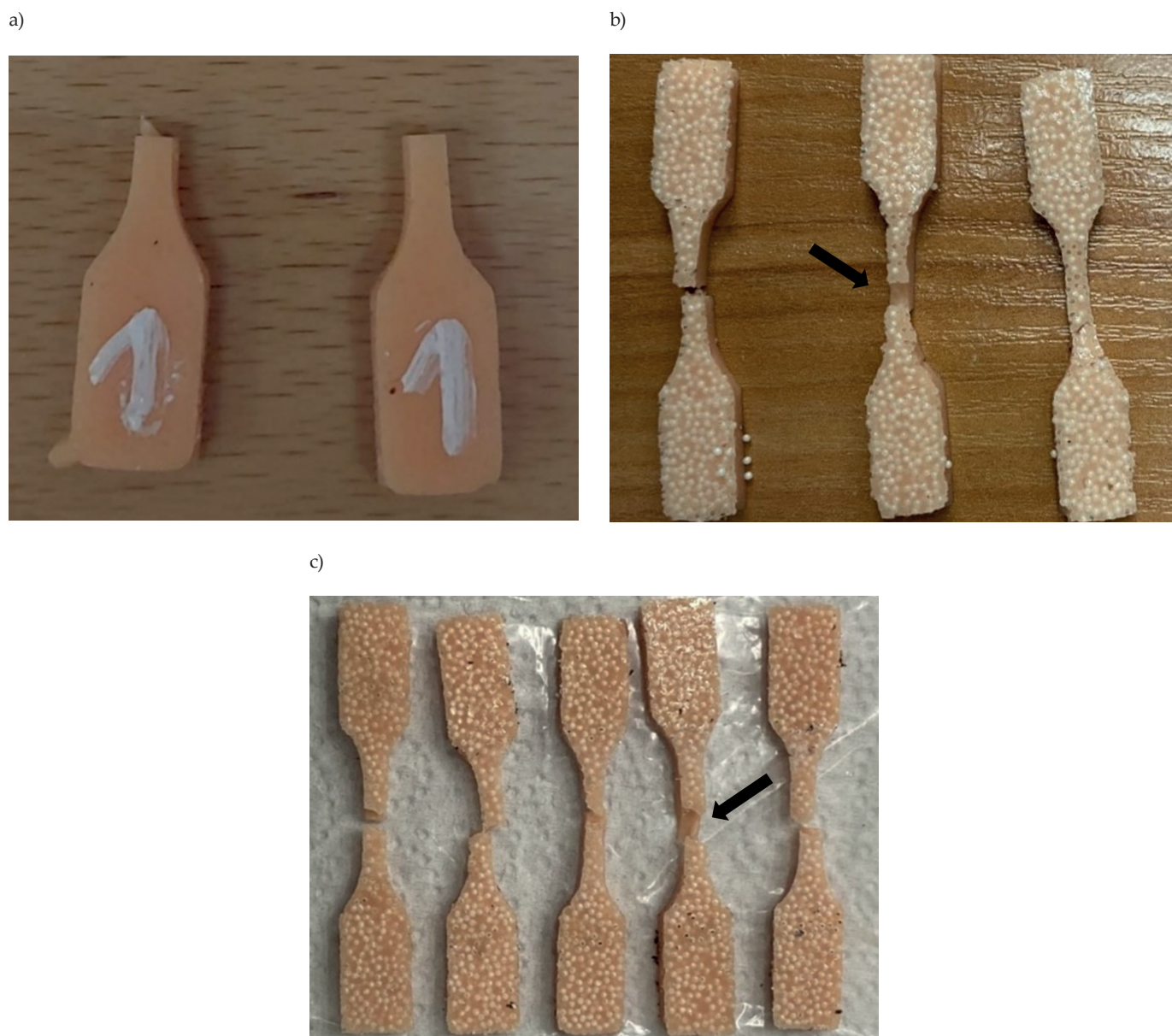
Fig. 4. Tensile testing samples: reference material (a), unaged (b) and aged (c) composites – the arrows indicate the samples' fracture
