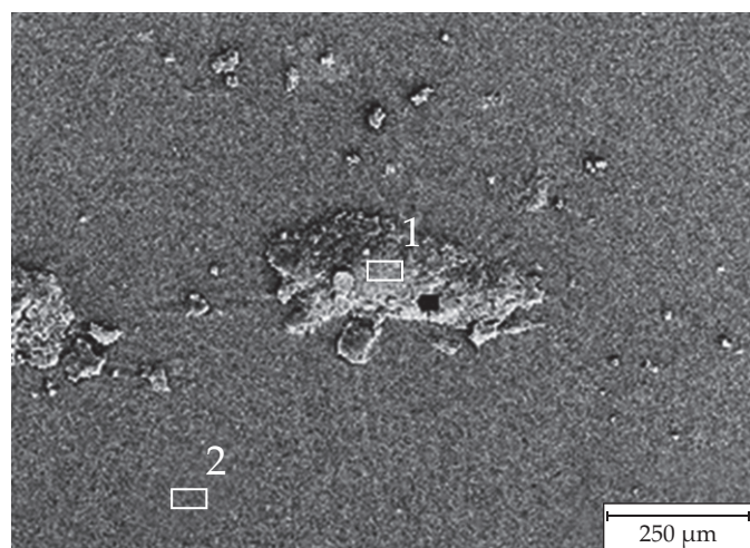
Fig. 8. EDS analysis areas: adhered substance (1) and silicone matrix (2)
