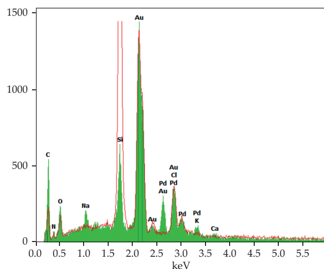
Fig. 9. EDS of adhered substance (green graph) and silicone matrix (red graph)
