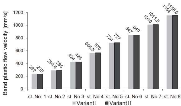
Fig. 7. Band plastic flow velocity changes obtained during numerical simulation of the continuous rolling process of the round bars of 70 mm in diameter from feedstock according to variant I and II
