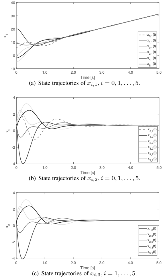
Fig. 3. State trajectories of heterogeneous systems.
