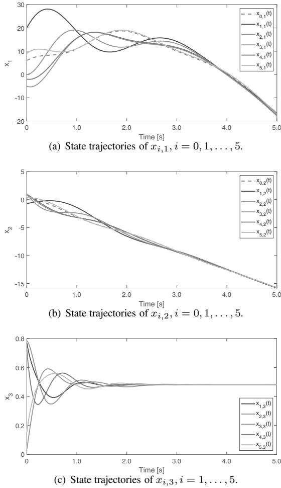
Fig. 2. State trajectories of homogeneous systems.
