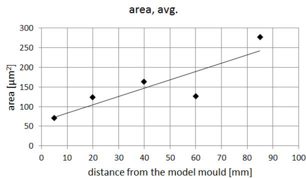
Fig. 2. The average size of carbides on perpendicular sections
