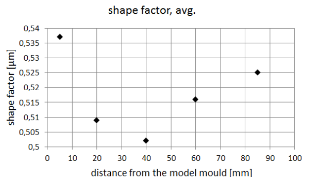
Fig. 11. The average shape factor of carbides on parallel sections
