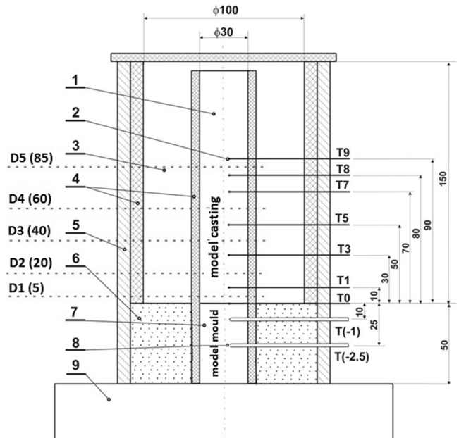
Fig. 1. Construction of the ATD-Is100 tester with indicated position of thermocouples and specimens used in the analysis, 1 – model casting, 2 – S-type thermocouple, 3 – thermal insulator, 4 – insulating material Sibral 300, 5 – steel casing, 6 – moulding material (quartz sand), 7 – model mould, 8 – K-type thermocouple, 9 – base, T0 – S-type thermocouple located on the border of the model casting – model mould, T1 ÷ T9 – S-type thermocouples placed in the model casting [2]
