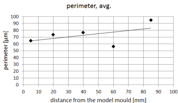
Fig. 3. The average perimeter of carbides on perpendicular sections
