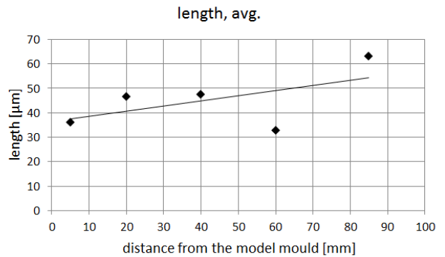
Fig. 9. The average length of carbides on parallel sections
