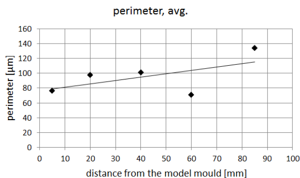
Fig. 8. The average perimeter of carbides on parallel sections
