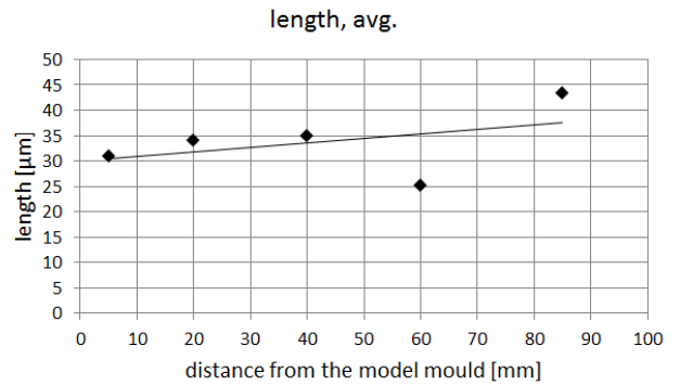
Fig. 4. The average length of carbides on perpendicular sections
