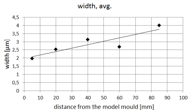
Fig. 10. The average width of carbides on parallel sections
