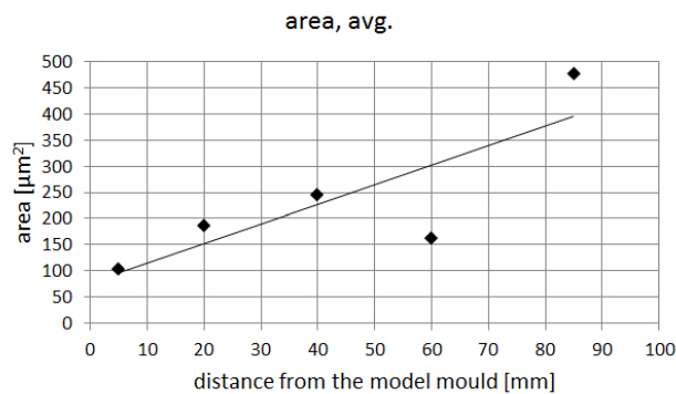
Fig. 7. The average size of carbides on parallel sections
