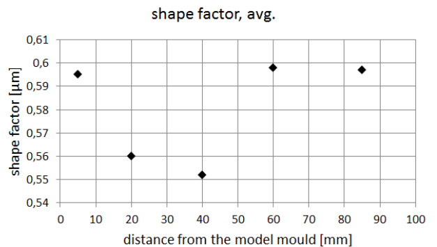
Fig. 6. The average shape factor of carbides on perpendicular sections
