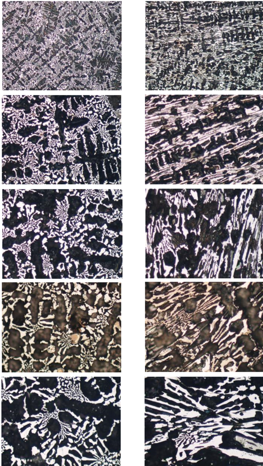
Fig. 12. Microstructure on perpendicular (left) and parallel (right) sections to the direction of heat removal distant from the model mould of 5, 20, 40, 60, 85 [mm], mag. 200x, etched
