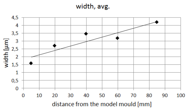
Fig. 5. The average width of carbides on perpendicular sections
