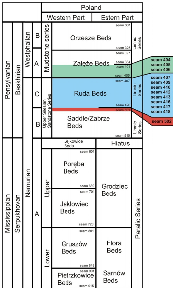
Fig. 2. A stratigraphic table of the carboniferous rocks of USCB, modified after Weniger et al. (2012). The color denotes the formations and coal seams from which research samples were collected
