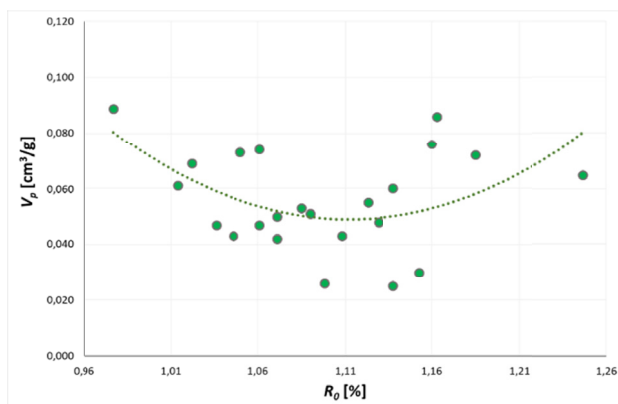
Fig. 8. Impact of the degree of coalification on the micropore volume
