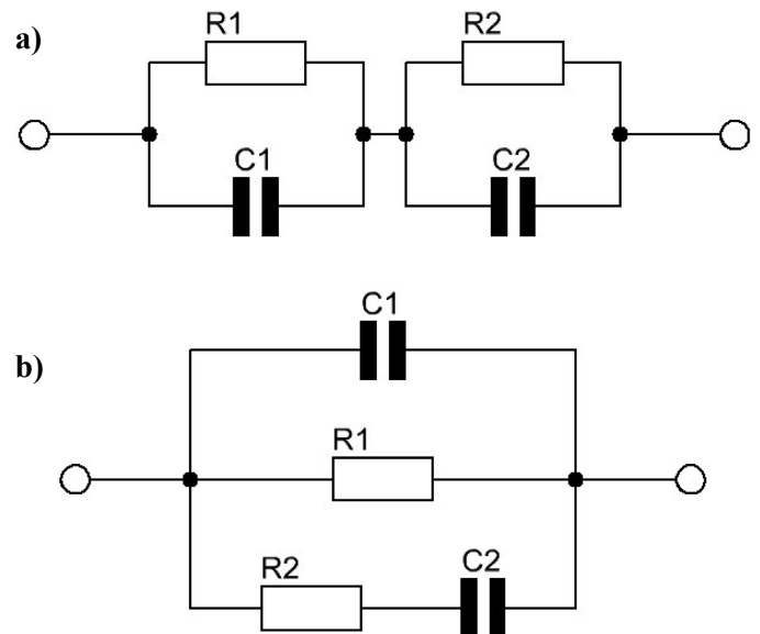
Fig. 5. The electrical equivalent circuits of the same impedance: (a) the Voigt's circuit, [(R_1C_1)(R_2C_2)] ; (b) the Maxwell's circuit (R_1C_1[R_2C_2])
