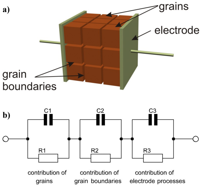
Fig. 1. Brick-layer model of ceramics (a) and corresponding electric equivalent circuit (R_1C_1)(R_2C_2)(R_3C_3) (b)
