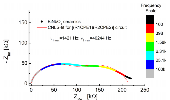
Fig. 6. Impedance data plotted in a complex Z'' - Z' plane (circles) and CNLS fit (line) calculated according to a Voigt's equivalent circuit [(R_1CPE_1)(R_2CPE_2)]
