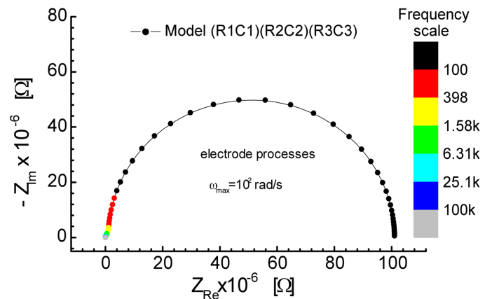
Fig. 3. Theoretical impedance response of a circuit (R_1C_1)(R_2C_2)(R_3C_3) exhibiting similar capacitive components and different resistance components plotted on a complex Z''-Z' plane
