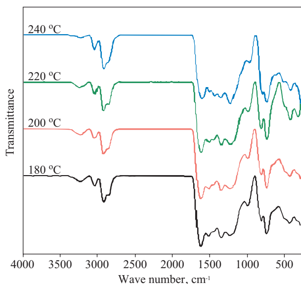
Fig. 7. FT-IR spectra of monomer M-A after different thermal treatment
