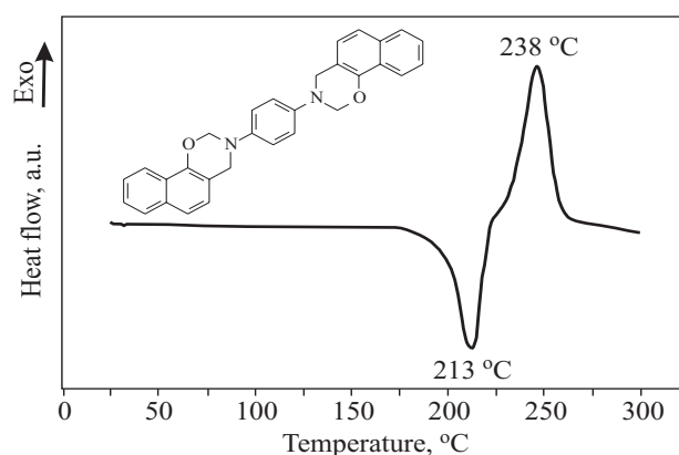
Fig. 6. DSC thermogram of M-B
