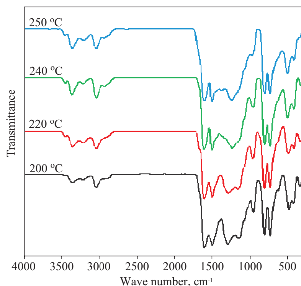
Fig. 8. FT-IR spectra of monomer M-B after different thermal treatment
