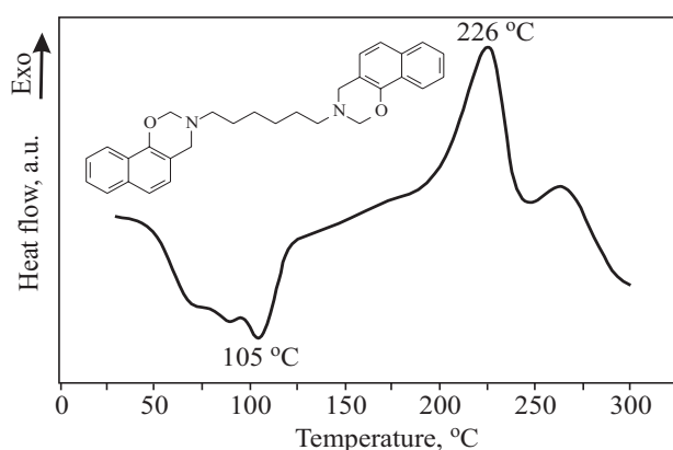
Fig. 5. DSC thermogram of M-A
