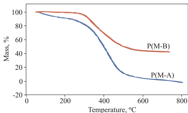
Fig. 9. TGA curves of polynaphthoxazines P(M-A) and P(M-B)
