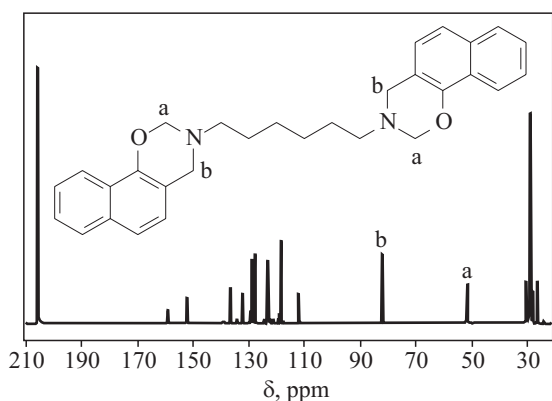
Fig. 4. ^{13}\text{C} NMR spectrum of M-A
