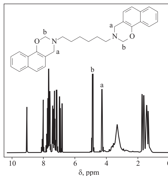
Fig. 3. 1 H NMR spectrum of M-A
